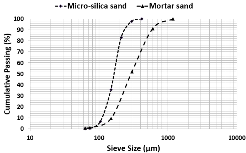
Figure 1: Grain size distribution of Silica Sand (SS) and Mortar Sand (MS)
