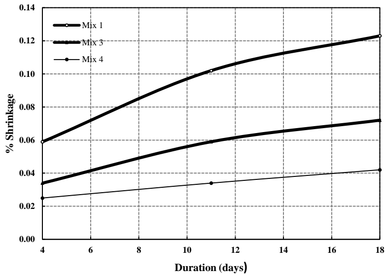
Figure 7: Shrinkage test results
