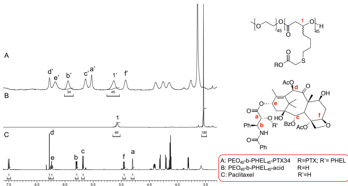
Figure 2.4. ^1\text{H} NMR spectra of a) PEO 45 - b -PHEL 45 -PTX34, b) PEO 45 - b -PHEL 45 -acid, and c) free paclitaxel. The peaks labeled with ‘ indicate peaks corresponding to conjugated molecules.
