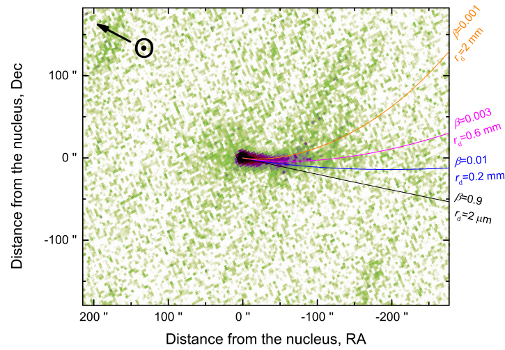
Figure 1.8 Syndyne diagram of a comet. Reproduced from Figure 1 of Ye & Wiegert (2014).
