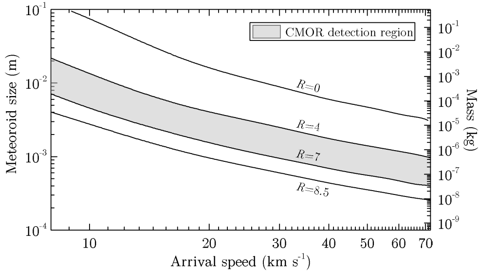
Figure 4.1 Size-speed relation of meteors as a function of absolute magnitude in the general R = 0 (typical detection limit of all-sky video networks), R = 4 (typical detection limit of narrow field video networks, as well as the upper limit of automated radar detection as meteor echo scattering changes from the underdense to the overdense regime, c.f. Ye et al., 2014), R = 7 (CMOR median for meteor orbits) and R = 8.5 (CMOR detection limit) assuming bulk density of 1000 \text{ kg m}^{-3} . Calculated using the meteoroid ablation model developed by Campbell-Brown & Koschny (2004), where the luminous efficiency is constant at 0.7% and the ionization coefficient is from Bronshten (1981). Note that other authors (Jones, 1997; Weryk & Brown, 2013) have argued that these coefficients may be off by up to a factor of \sim 10 at extreme speeds ( v_g \lesssim 15 \text{ km s}^{-1} or v_g \gtrsim 70 \text{ km s}^{-1} ), but most of the showers we examined in this work have moderate v_g , hence this issue does not impact our final results. The CMOR detection range is appropriated to an ionization coefficient I of 5–100 in Wiegert et al. (2009)’s model.
