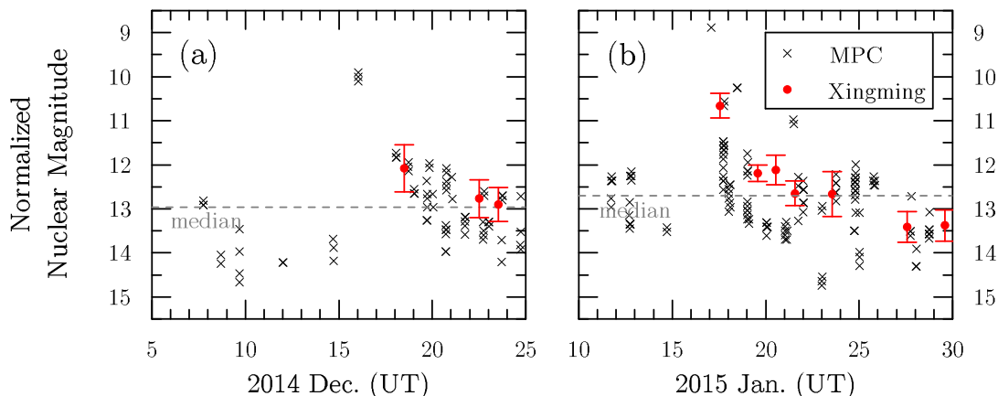
Figure 2.1 Nucleus magnitude of 15P/Finlay around the time of (a) the first outburst, and (b) the second outburst. The Minor Planet Center (MPC) magnitudes (plotted in crosses) are extracted from the Observations Database on the MPC website. The Xingming magnitudes (plotted in red dots) are derived from the monitoring observations by the Xingming 0.35-m telescope with aperture radius \rho = 5000 km. The magnitudes are normalized to \Delta = r_h = 1 AU assuming a brightening rate n = 4 (Everhart, 1967).
