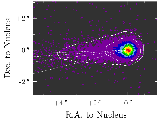
Figure 3.1 The 2014 Apr. 9 GMOS-N image (stretched in logarithmic scale) superimposed with the synchronic model. The ages of the synchronic lines (dashed lines) are (in counterclockwise order) 10, 25, 50 and 100 d respectively. The oldest visible dust was released at \tau \sim 50 d, appropriate to late Feb. 2014.
