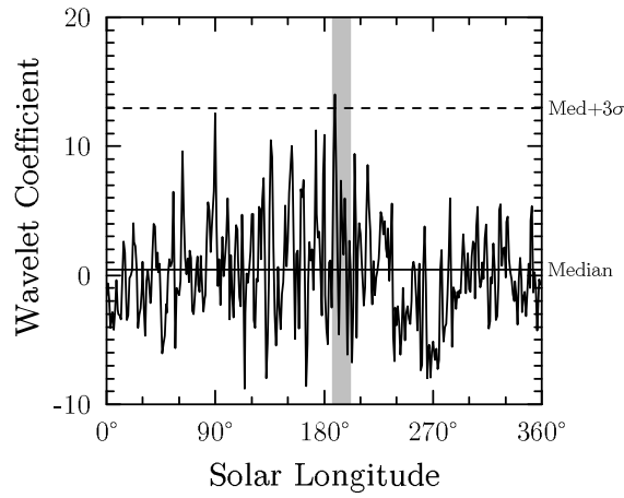
Figure 2.7 The variation of the wavelet coefficient at the calculated Finlayid radiant \lambda - \lambda_{\odot} = 66^{\circ} , \beta = -25^{\circ} , v_G = 13 \text{ km} \cdot \text{s}^{-1} using the stacked “virtual year” CMOR data. The shaded area is the expected time window for Finlayid activity (solar longitude \lambda_{\odot} \sim 193^{\circ} ).
