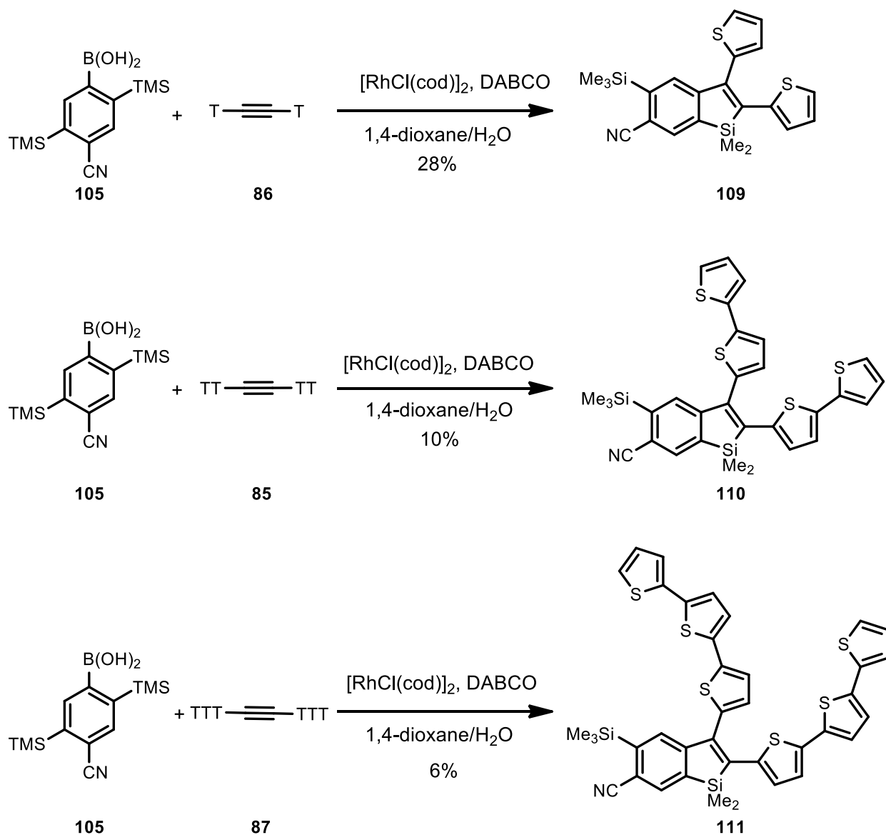
Scheme 25 Synthesis of nitrile substituted benzosiloles.
