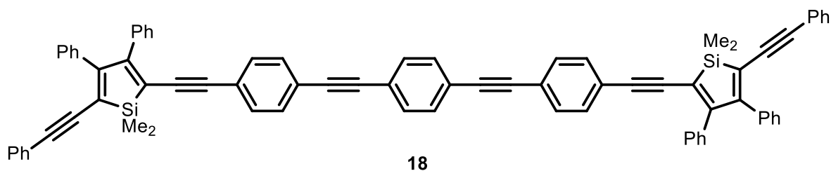
Figure 6 Extended silole chromophores.
