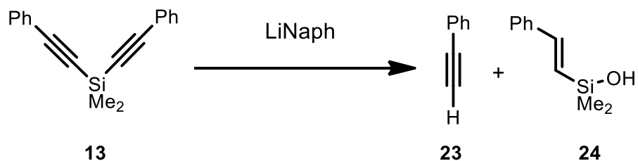
Scheme 1 Byproducts formed as a result of unknown impurities in the lithium naphthalenide.
