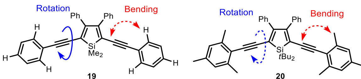
Figure 8 The steric rigidity of 2,5-arylene ethynylenes.
