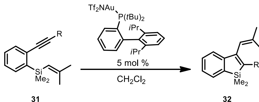
Scheme 4 Murakami's approach to 3-allylbenzosiloles using a gold catalyst.
