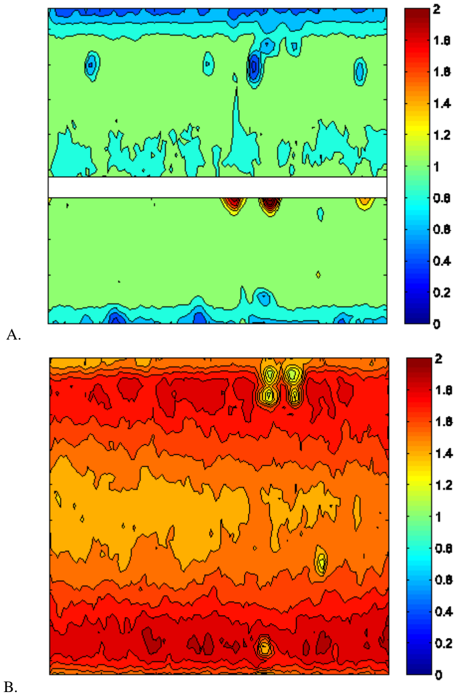
Figure 4.7: Vertical RMS velocity contour maps for conditions of buoyancy-inertia ratio of A) 0.002, and B) 0.0003 with colour bar units of [mm/s]
