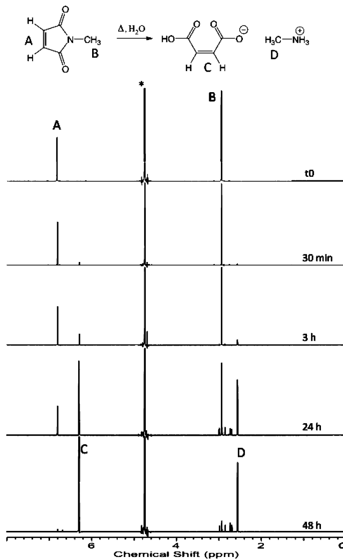
Figure 2.3: ^1H NMR spectrum recorded in D_2O showing the kinetics of hydrolysis of N -methylmaleimide. Peaks A and B are relative to the reactant, and peaks C and D are relative to the main products. * is the H_2O signal.
