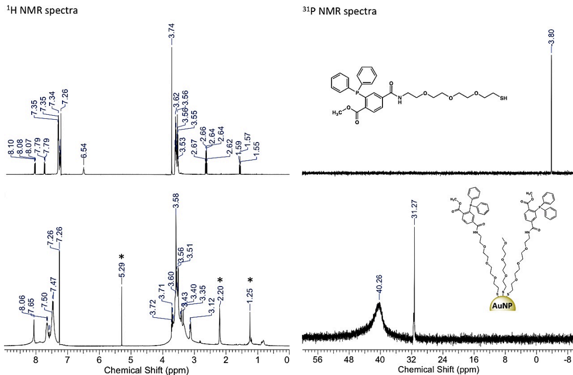
Figure 9.1: ^1\text{H} (left) and ^{31}\text{P} (right) NMR spectra of phosphine-thiol (4) (top) versus Staudinger-AuNP (bottom). *Denotes residual solvent peaks. Spectra calibrated against residual chloroform and \text{H}_3\text{PO}_4 .
