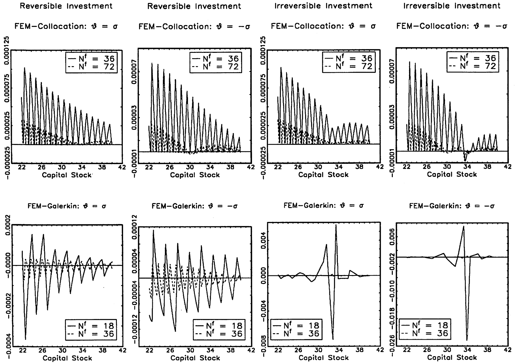
Figure 2b. Euler residuals for FEM-collocation and FEM-Galerkin
