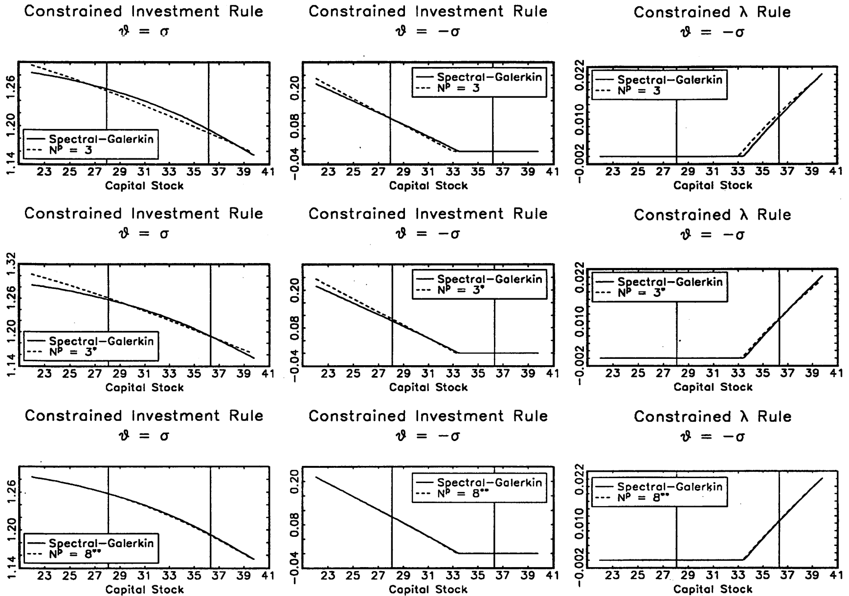
Figure 5. PEA versus Spectral-Galerkin Investment and Lambda Rules in the Irreversible Investment economy
