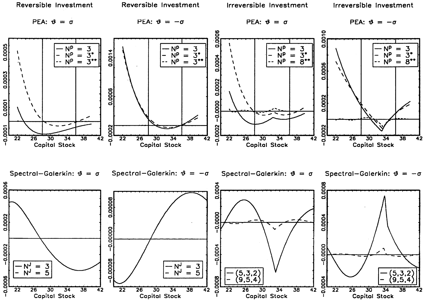
Figure 2a. Euler residuals for PEA and Spectral-Galerkin
