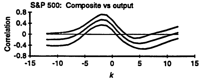
Figure 5: Correlation Between Stock Price Measure at t and Output at t-k Price and output data logged and detrended by HP filter
