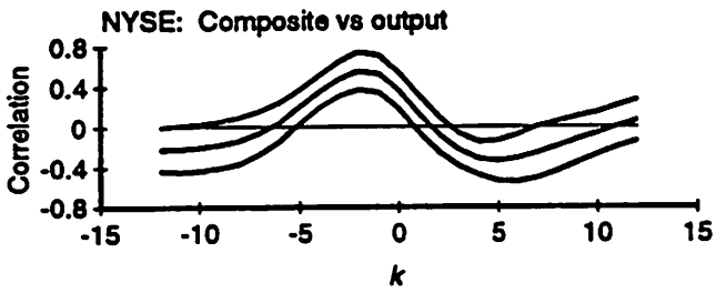
Figure 5: Correlation Between Stock Price Measure at t and Output at t-k Price and output data logged and detrended by HP filter
