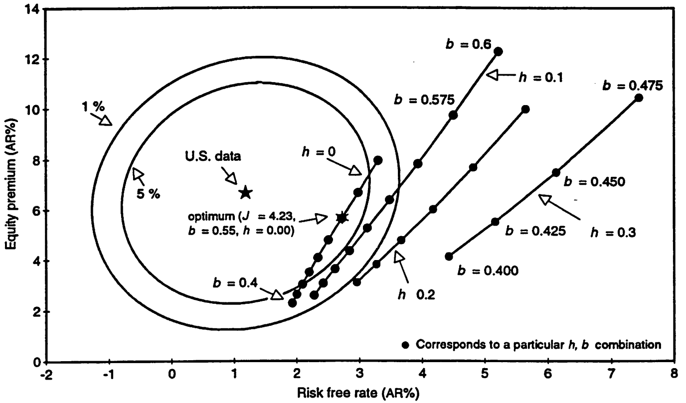
Figure 6: Assigning Values to Preference Parameters, b and h
