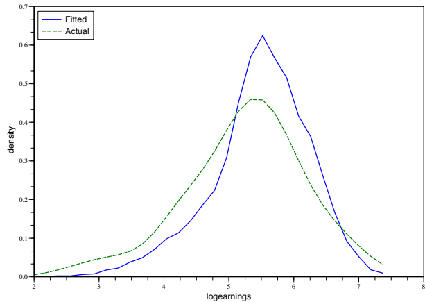
Densities of fitted and actual log present value of earnings for period 6 for overall sample
