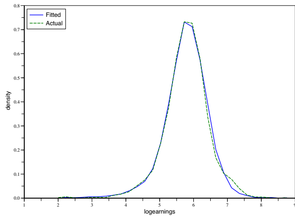
Densities of fitted and actual log present value of earnings for period 3 for overall sample
