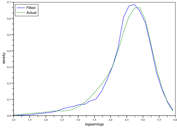
Densities of fitted and actual log present value of earnings for period 1 for overall sample
