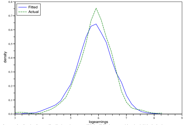
Densities of fitted and actual log present value of earnings for period 4 for overall sample
