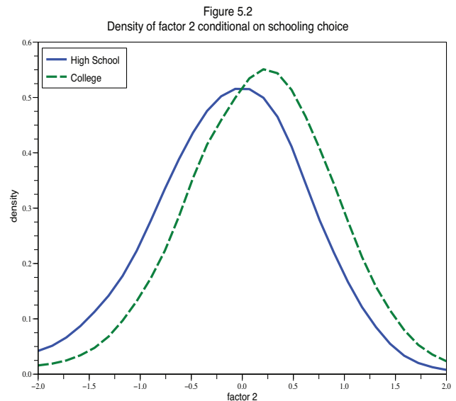
Let f(\theta) denote the density function of factor \theta , f(\theta) is allowed to be a mixture of normals. The solid line plots the density of the factor conditional on choosing high school, that is, f(\theta|choice=high\ school) . The dashed line plots the density of the factor conditional on choosing college, that is, f(\theta|choice=college) . The plots are smoothed using a Gaussian kernel.
