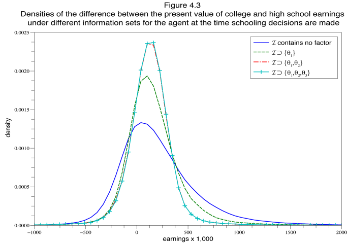
Let Y_H, Y_C denote the present value of high school and college earnings from age 18 to 65 discounted at a 3% interest rate respectively. Define G = Y_C - Y_H . Let \mathcal{I} denote the agent's information set and f(g|\mathcal{I}) denote the density of the present value of earnings conditional on the information set \mathcal{I} . The graph shows f(g|\mathcal{I}) with \mathcal{I} containing no factors, factor 1, factors 1 and 2, and all three factors. The plots are smoothed using a Gaussian kernel.
