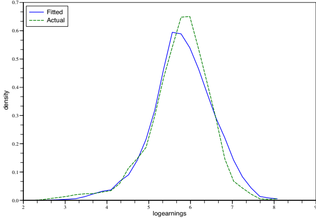
Densities of fitted and actual log present value of earnings for period 5 for overall sample
