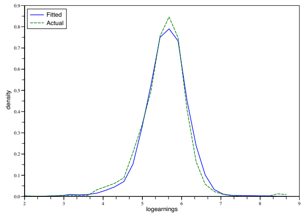
Densities of fitted and actual log present value of earnings for period 2 for overall sample
