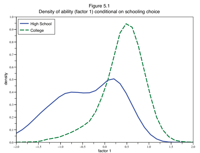
Let f(\theta) denote the density function of factor \theta , f(\theta) is allowed to be a mixture of normals. The solid line plots the density of the factor conditional on choosing high school, that is, f(\theta|choice=high\ school) . The dashed line plots the density of the factor conditional on choosing college, that is, f(\theta|choice=college) . The plots are smoothed using a Gaussian kernel.
