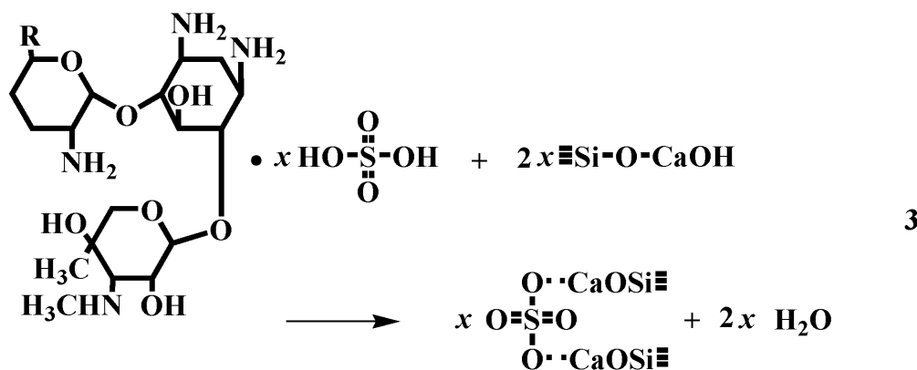
Scheme 5-2 Electrostatic interactions between Ca-OH groups and different drug molecules.
