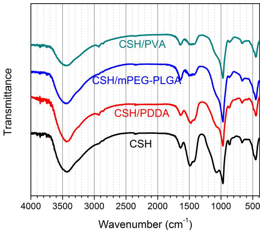
Figure 7-2 FTIR spectra of CSH nanosheets, and different CSH/polymer composites.
