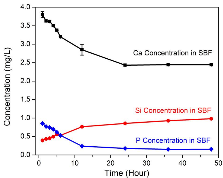
Figure 6-13 Concentration changes of Ca, P and Si after soaking CSH-IBU in SBF for different period of time.
