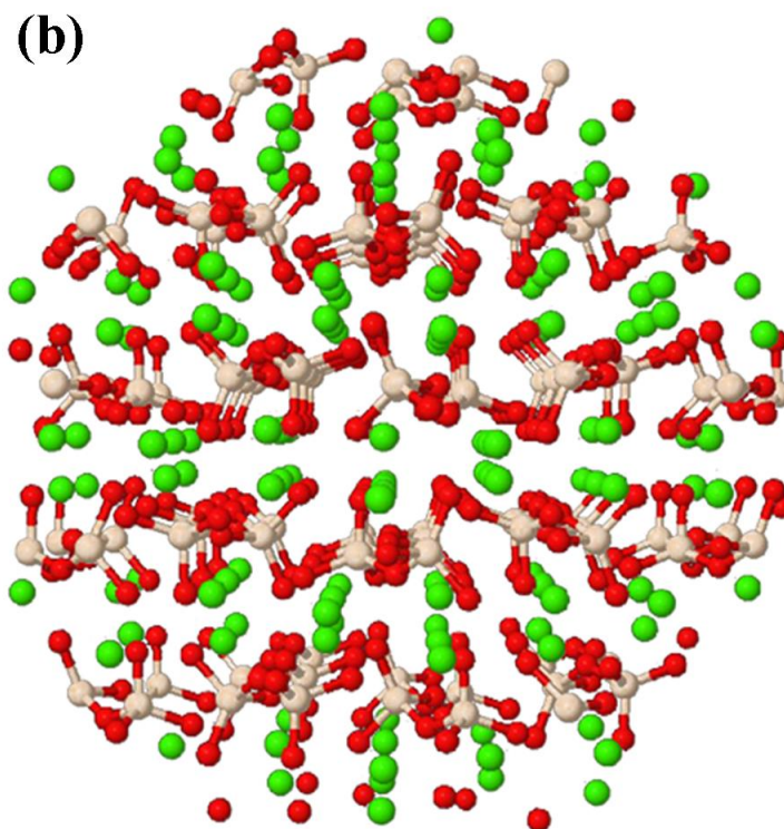
Figure 3-3 (a) TEY XANES spectra of calcium silicate hydrate and anhydrous calcium silicate carriers with different morphologies, comparison with FEFF calculation; (b) Crystal structure of rankinite simulated by FEFF (green, red and beige spheres stand for Ca, O and Si atoms, respectively).
