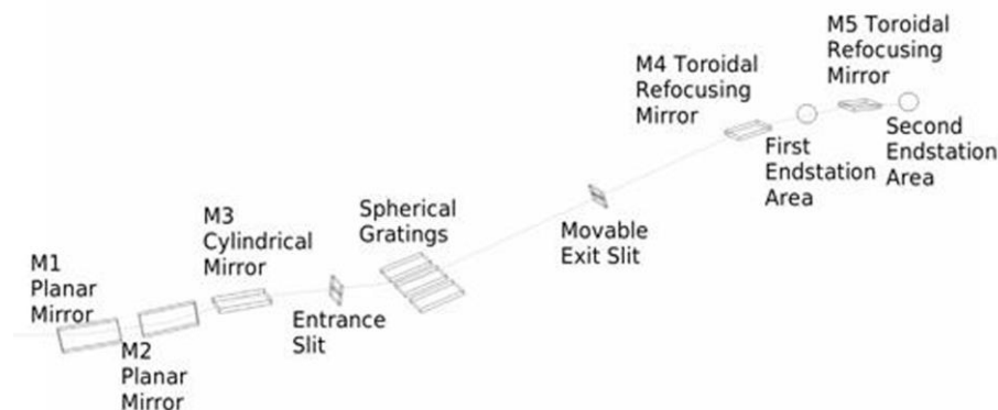
Figure 2-2 Layout of SGM beamline at CLS [6].
