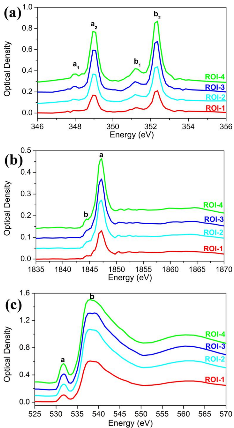
Figure 4-7 XANES spectra of individual CSH microspheres after IBU loading at Ca L_{3,2} -edge (a), Si K-edge (b) and O K-edge (c). (ROI 1-4 are the same regions as shown in Fig. 4-6(d)).
