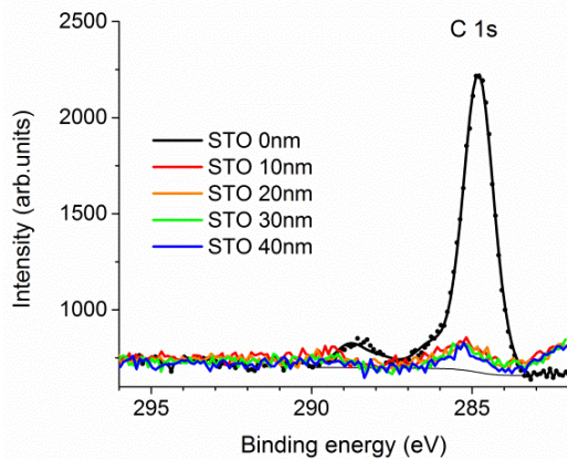
Figure 4.19. XPS 1s C peaks of STO crystal collected at surface and after sputtering at depth 10nm, 20 nm, 30 nm and 40 nm.
