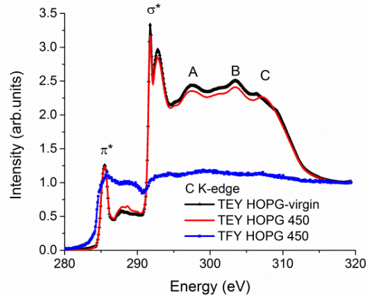
Figure 6.7. C K-edge TEY spectra of un-implanted graphite samples: virgin HOPG and annealed at 450°C; C K-edge TFY spectrum of HOPG annealed at 450°C is also shown. The flattened out spectral feature in TFY results from saturation (sample is optically thick).
