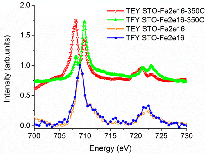
Figure 5.5. Fe L_{3,2} -edge XANES spectra of STO-Fe2e16 and STO-Fe2e16-350C collected in total fluorescence yield and in total electron yield.
