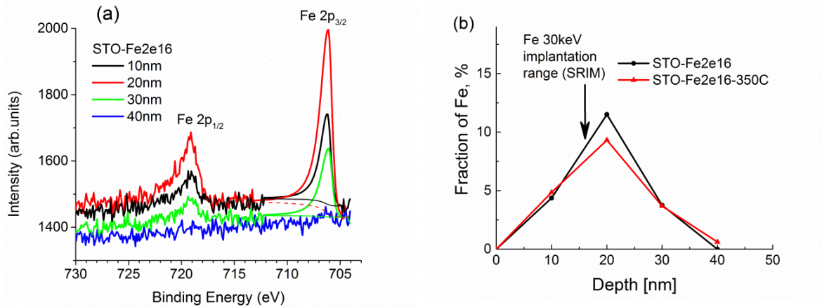
Figure 4.15 (a) XPS Fe 2p peaks for STO-Fe2e16 sample collected at 10 nm, 20 nm, 30 nm and 40 nm depth after sputtering. (b) Depth distribution of implanted Fe derived from the intensities of Fe 2p XPS peaks.
