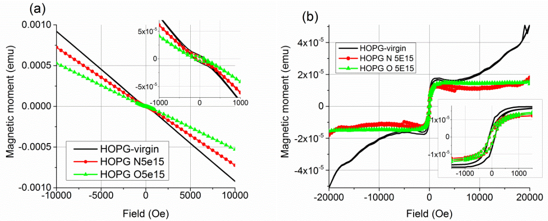
Figure 7.14. Magnetic moment of HOPG samples: (a) before and (b) after subtraction of the diamagnetic contribution. Inserts show enlarged image of hysteresis part.
