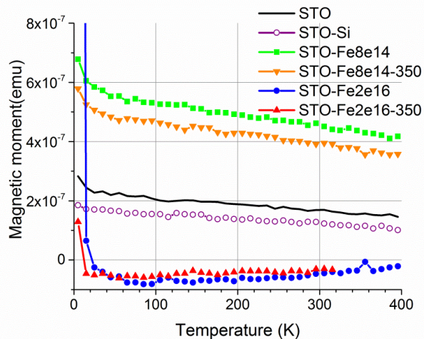
Figure 7.13. Remanent magnetization of STO samples.
