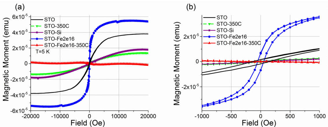
Figure 7.11 Magnetic moment ( M ) vs. field ( H ) curves of un-implanted STO and STO-350, Fe implanted samples STO-Fe2e16 and STO- Fe2e16-350C, and Si implanted STO after subtraction of diamagnetic contribution.
