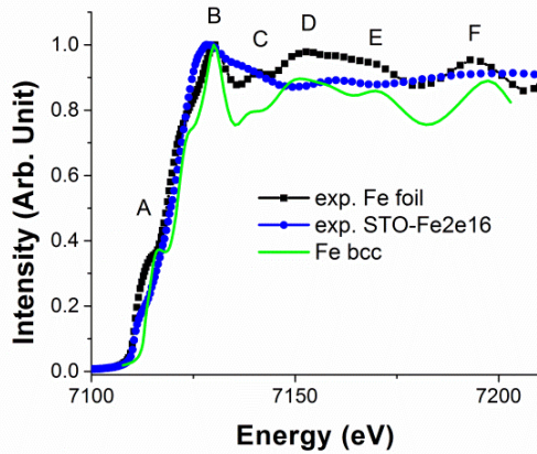
Figure 5.8. Experimental Fe K-edge XANES of STO-Fe2e16 and Fe foil and FEFF calculations for Fe foil with bcc unit cell.
