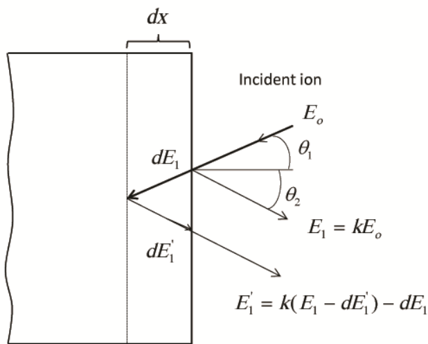
Figure 2.5 Schematic of of the energy loss processes in a thin layer.
