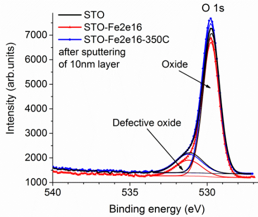
Figure 4.17. XPS 1s O peaks of STO crystal, implanted STO-Fe 2 e 16 and implanted and annealed STO-Fe 2 e 16 -350C samples collected after sputtering of 10nm layer.
