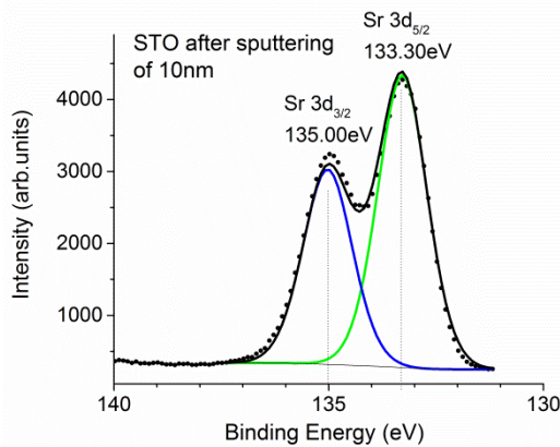
Figure 4.14. Sr 3d peaks in XPS spectra of STO crystal after sputtering of 10nm layer.
