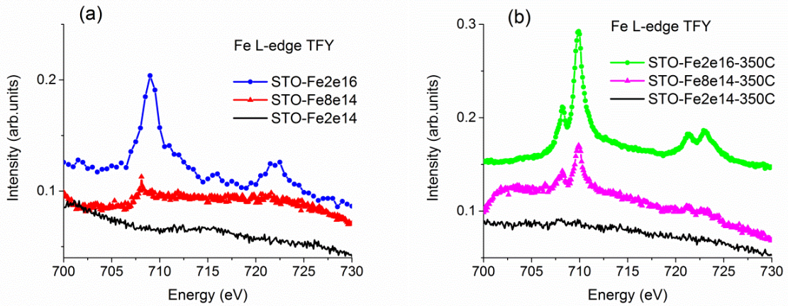
Figure 5.4. (a) Fe L_{3,2} -edge XANES spectra of STO implanted with different Fe^+ doses; (b) Fe L_{3,2} -edge XANES spectra of STO implanted with different doses and annealed, collected at the total fluorescent yield.
