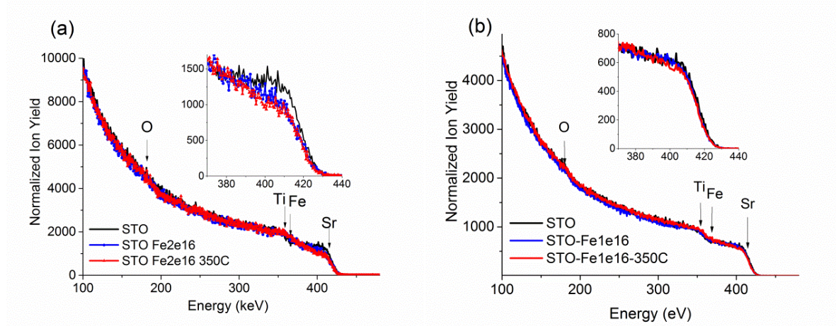
Figure 4.8. RBS spectra of (a) STO, STO-Fe2e16 and STO-Fe2e16-350C samples; and (b) STO, STO-Fe1e16 and STO-Fe1e16-350C samples collected in random geometry with 0.5 MeV He + beams.
