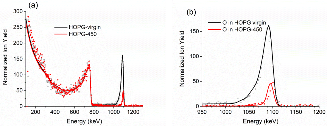
Figure 6.2. (a) RBS spectra for virgin HOPG and HOPG annealed in vacuum at 450°C collected with 3.03 MeV He + beams; (b) Magnified oxygen peak.
