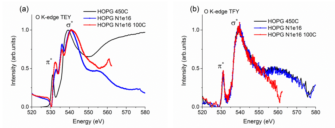
Figure 6.13 O K-edge XANES of un-implanted HOPG, HOPG-N1e16 and HOPG-N1e16-100C samples collected in (a) total electron yield and (b) inverted fluorescence yield.
