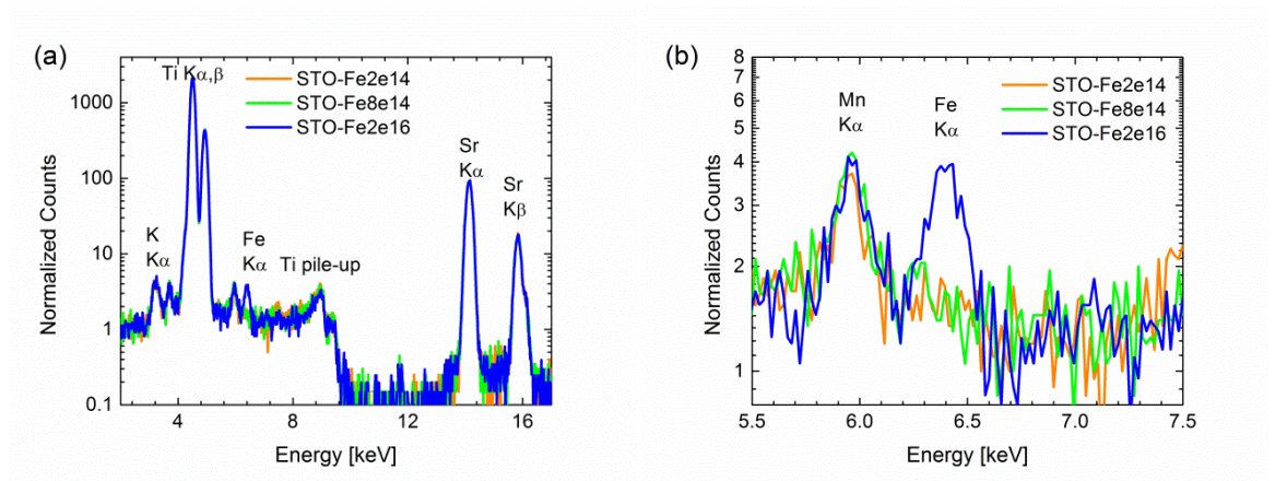
Figure 4.4. (a) PIXE spectra of Fe implanted samples STO-Fe2e14, STO-Fe8e14 and STO-Fe2e16. (b) Enlarged image of Fe K \alpha and Mn K \alpha peaks.
