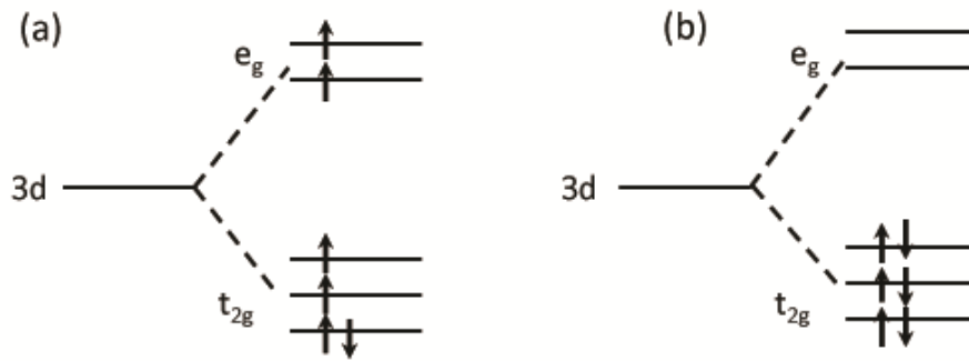
Figure 7.2. 3d electron level of \text{Fe}^0 ( [\text{Ar}] 3d^6 4s^2 ): (a) “high” spin configuration, (b) “low” spin configuration.
