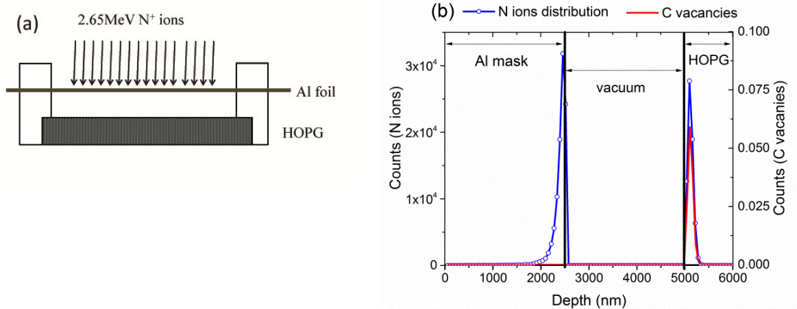
Figure 6.1. (a) Schematic of the implantation of 2.65 MeV N + in HOPG through Al mask; (b) SRIM simulation demonstrates distribution of N ions and C vacancies in HOPG.
