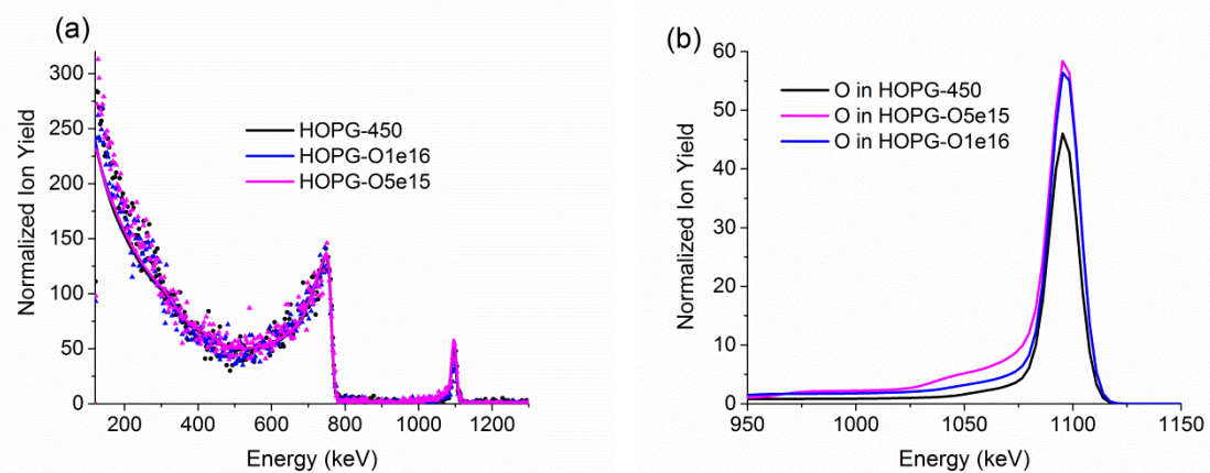
Figure 6.3. (a) RBS spectra recorded with He + beam at energy 3.03 MeV for HOPG-450, HOPG-O1e16 and HOPG-O5e15 samples; (b) Magnified oxygen peak.
