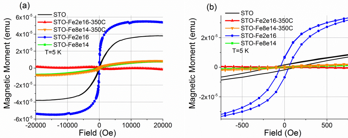
Figure 7.12 (a) Magnetic moment (M) vs. field (H) curves of un-implanted STO and STO implanted different Fe doses after subtraction of diamagnetic contribution; (b) enlarged part with ferromagnetic hysteresis.
