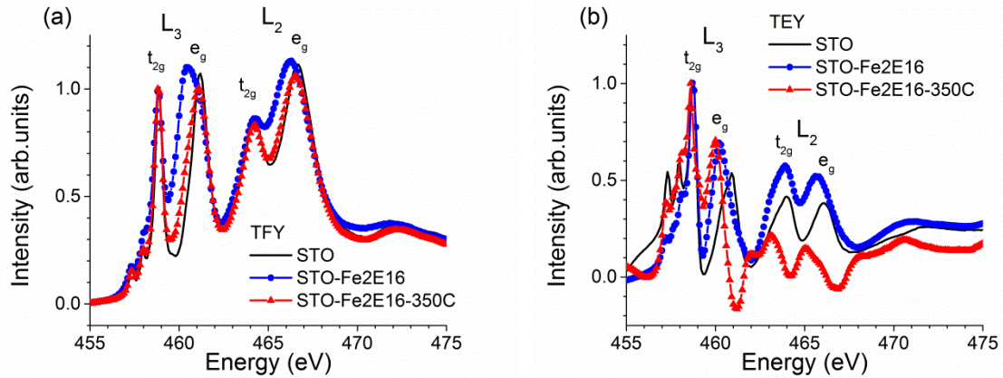
Figure 5.2. Ti L 3,2 -edge XANES spectra of virgin STO, STO-Fe 2 e16 and STO-Fe 2 e16-350C samples: (a) collected in total fluorescence yield; (b) collected in total electron yield.
