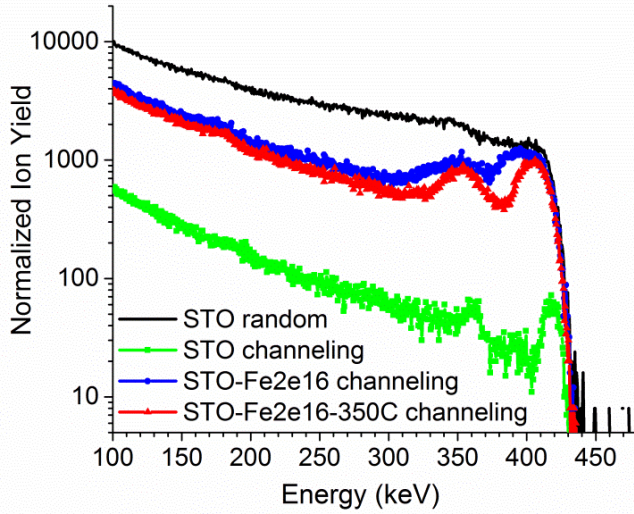
Figure 4.9. RBS spectra of STO, STO-Fe2e16 and STO-Fe2e16-350C samples collected in channeling geometry with 0.5 MeV He + beams.
