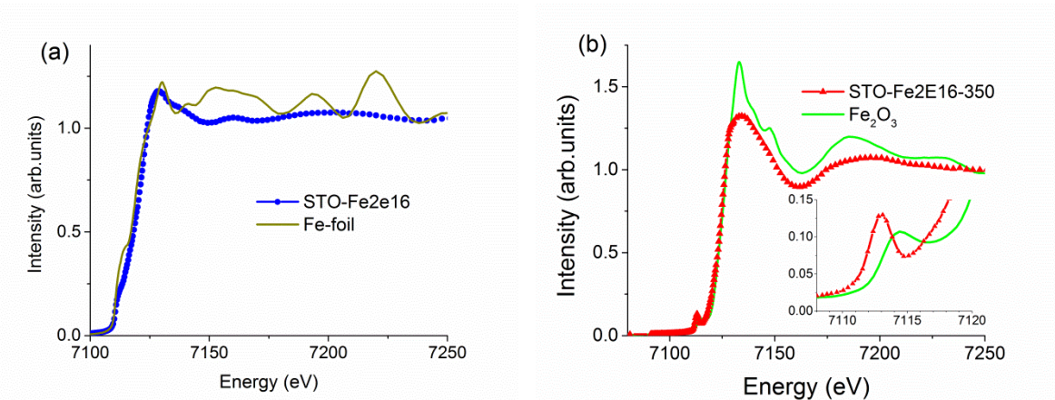
Figure 5.3. Fe K-edge TEY XANES spectra of STO samples: (a) implanted sample STO-Fe 2 e16; (b) implanted and annealed sample STO-Fe 2 e16-350C. Iron foil and iron oxide Fe 2 O 3 spectra are shown for comparison.
