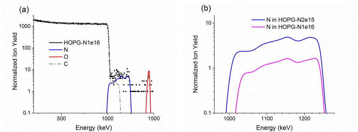
Figure 6.4. (a) RBS spectrum recorded He + beam at energy 3.7 MeV for N irradiated sample HOPG-N1e16; (b) Magnified peaks from N for HOPG-N1e16 and HOPG-N2e15 samples..
