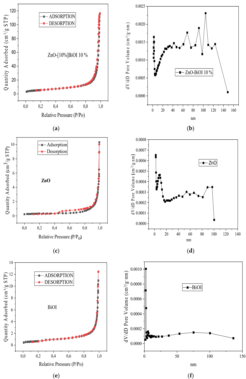
Figure 4. Textural properties (a) N 2 adsorption-desorption isotherm of ZnO-[10%]BiOI (b) Barret-Joyner-Halender (BJH) pore size distribution of ZnO-[10%]BiOI (c) N 2 adsorption-desorption isotherm of pristine ZnO (d) Barret-Joyner-Halender (BJH) pore size distribution of ZnO (e) N 2 adsorption-desorption isotherm of BiOI (f) Barret-Joyner-Halender (BJH) pore size distribution of BiOI.
