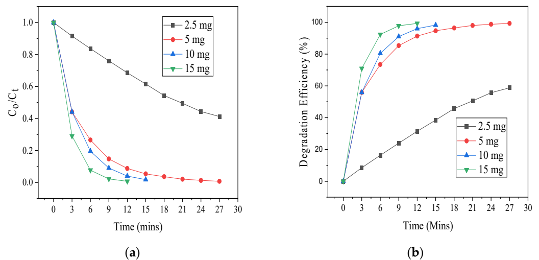
Figure 6. (a) Photodegradation of 40 ppm SCN - at varying initial ZnO-[10%]BiOI dosage (b) photodegradation efficiencies.
