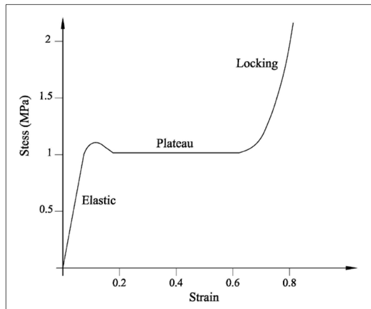
Figure 4.2: Typical compressive behavior of LPF
