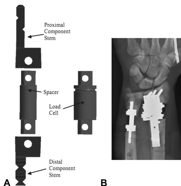
FIGURE 1: Distal ulna load cell system. A An exploded view of the instrumented distal ulna load cell. This implantable system comprises 4 parts: the distal component stem, the proximal component stem, the spacer, and the load cell. For surgical setup, a spacer was used (left); however, for testing purposes, this was removed and replaced with the instrumented load cell (right). B The distal implant system is shown in situ . Also visible is the distal radius malalignment implant.
