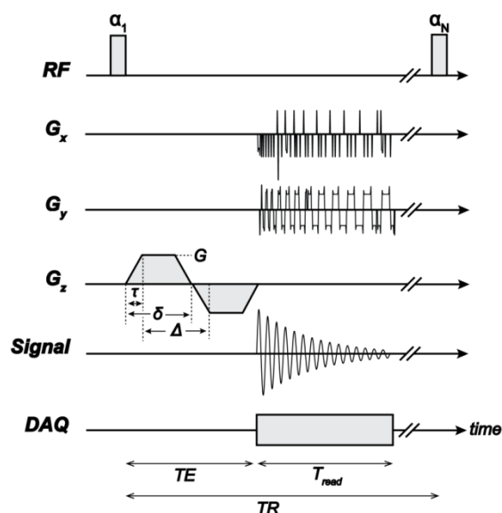
Figure 1-12: A diagram of the diffusion-weighted Sectoral pulse sequence including a bipolar trapezoidal gradient pulse with diffusion time, \Delta , lobe duration, \delta , ramp time, \tau , and gradient magnitude, G .
