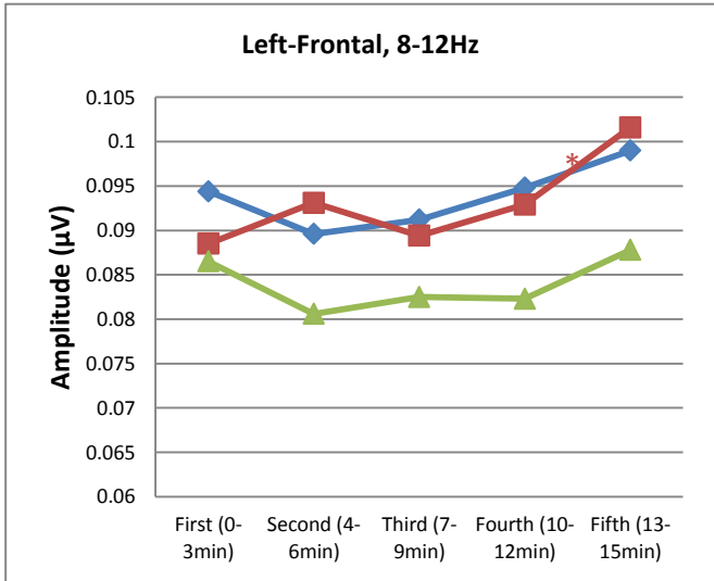
Figure 3: Within group differences in full-band EEG alpha amplitudes (8-12Hz) during 15-minute intervention across frontal and posterior sites
