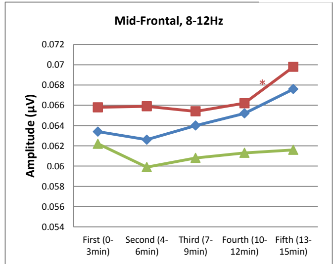
Figure 3: Within group differences in full-band EEG alpha amplitudes (8-12Hz) during 15-minute intervention across frontal and posterior sites
