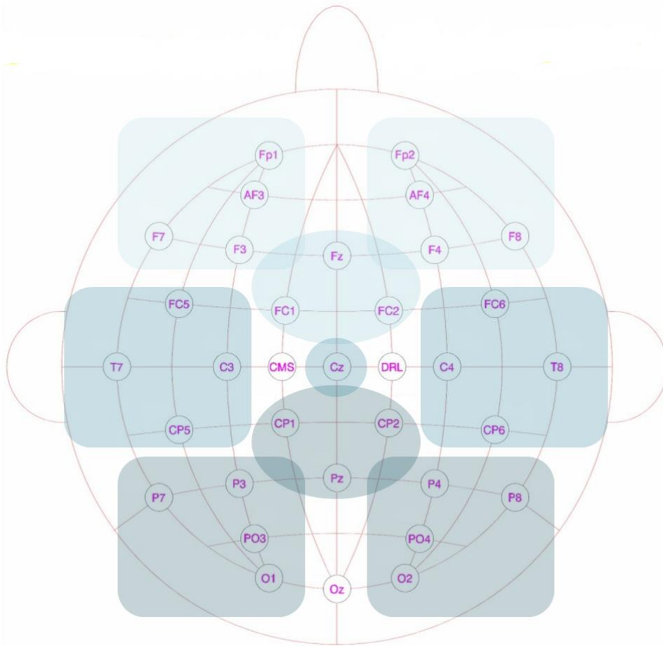
Figure 1: Topography of recorded EEG electrode positions, with shaded regions selected for statistical analyses
