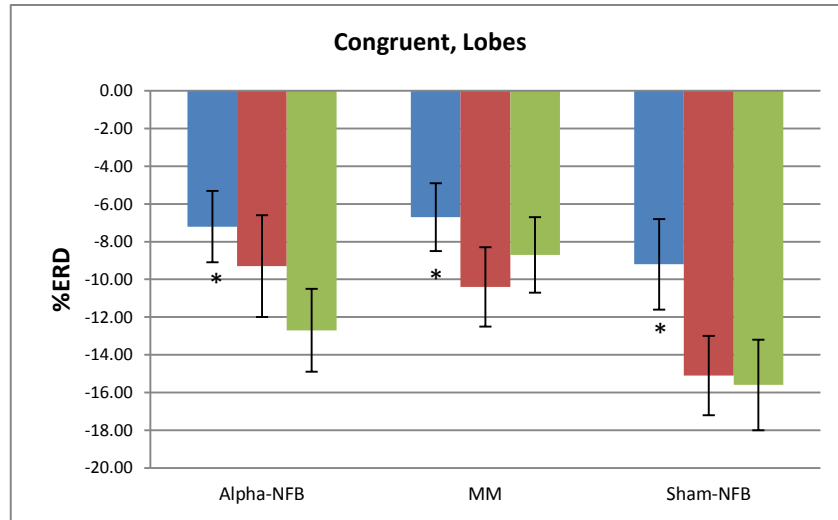
Figure 9: Lobe patterns of upper-band EEG alpha (10-12Hz) ERD during 400-600ms post-stimulus interval
