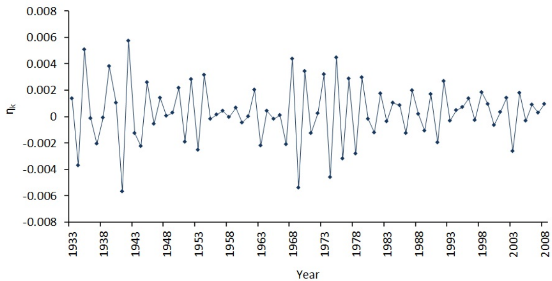
Figure 4.9: \eta_k process.
