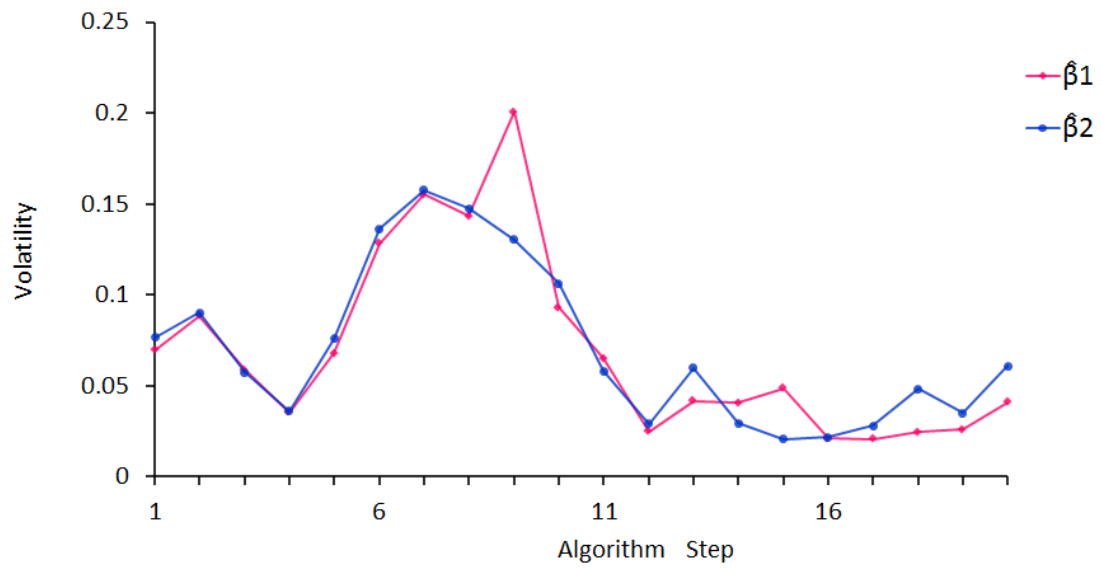
Figure 4.7: Evolution of \hat{\beta} under the 2-state setting.
