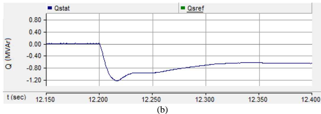
Figure 4.15 (a) Wind farm terminal voltage and (b) reactive power supplied by STATCOM when 4 turbines operational
