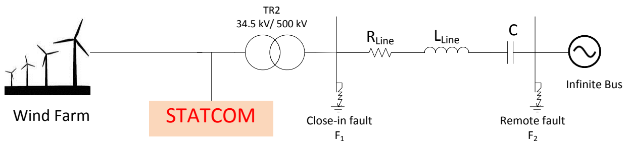
Figure 5.8 Study System 2 for fault analysis with STATCOM
