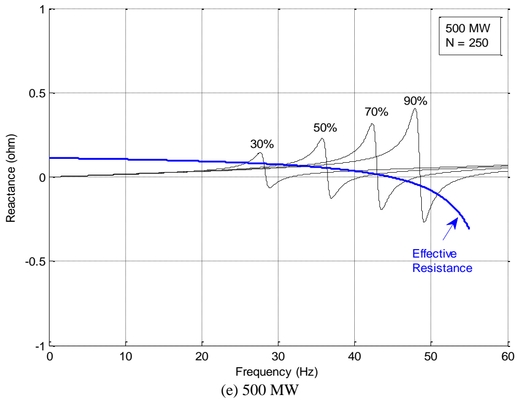
Figure 5.12 Equivalent reactances seen from the rotor for different sizes of single-cage induction generator based wind farms connected to Study System 1
