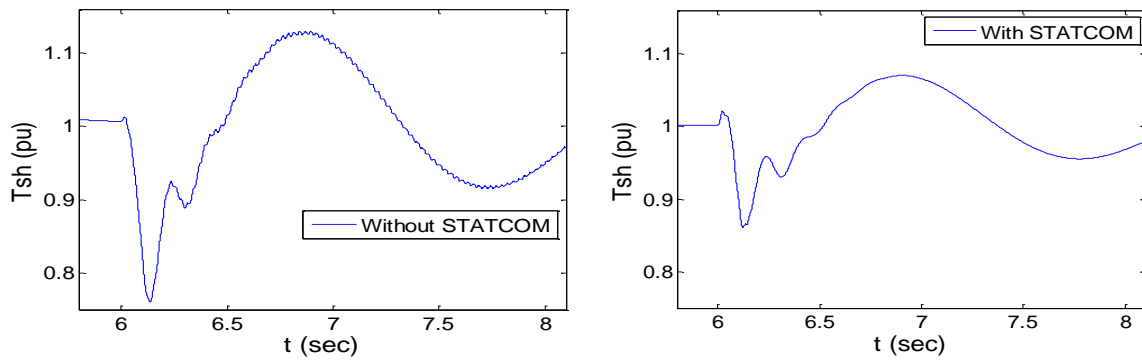
(c) Shaft torque
