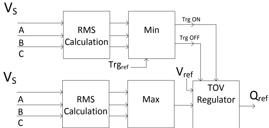
Figure 2.20 Block diagram of temporary overvoltage (TOV) regulator
