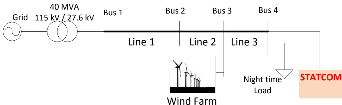
Figure 4.11 Single line representation of feeder network with wind farm and night time load
