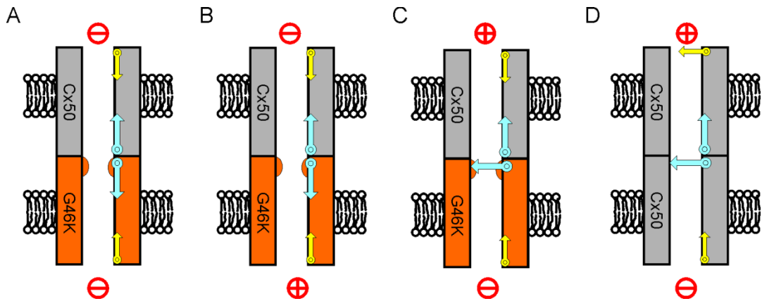
Figure 3.1 A possible mechanism for the abolished fast gating in Cx50/G46K heterotypic GJ channel. A) A cartoon diagram showing the profile of a heterotypic GJ channel docked by Cx50 (grey) and G46K (orange) hemichannels. Note that the TM1/E1 border is narrower in the G46K hemichannel than in the Cx50 hemichannel, indicating a physical and electrical barrier to ion flow. The channel keeps opening without V_j administration. B) Imposing positive V_j on the G46K side fails to close any gates because most V_j drop is imposed at the TM1/E1 border of the G46K hemichannel, but the loop gate at this location only responds to the intracellular negative potential. C) When applying sufficient negative V_j on the G46K side, loop gate of the G46K hemichannel is closed but fast gate of the Cx50 hemichannel cannot be shut down due to the low V_j drop on it. D) When the same V_j condition as in C) is applied on a homotypic Cx50 GJ channel, both fast gate of the top Cx50 hemichannel and loop gate of the bottom Cx50 hemichannel have a chance to be closed, but the fast gate is much more sensitive than the loop gate.
