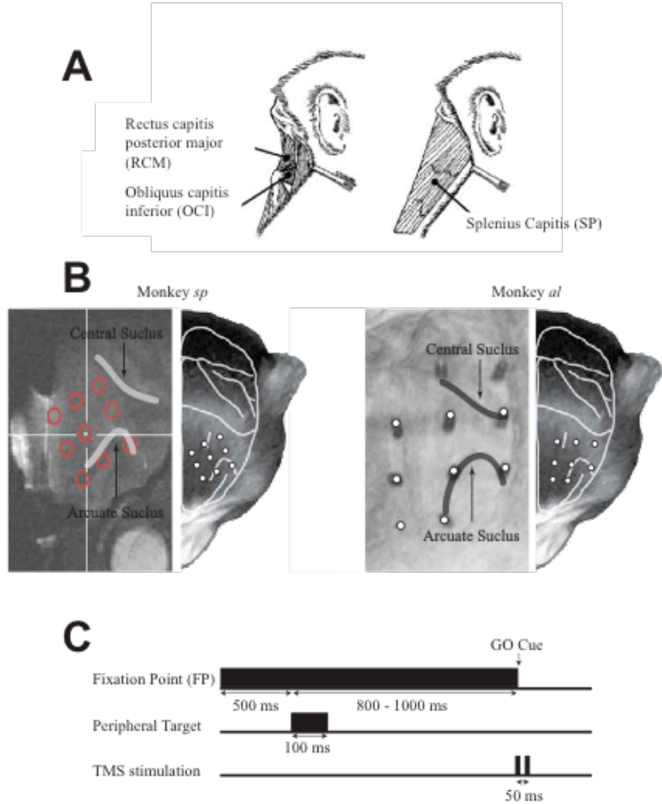
Figure 4: Methods
