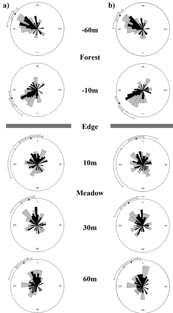
Figure 7. Rose diagrams show the distribution of (a) initial and (b) final divergence angles relative to the edge from all release points in the forest and meadow for P. glaucus . Data were collected at three selected sites in Norfolk County during May-July 2012. Points on the circle are the mean directions bounded by non-parametric confidence intervals. Females are represented by gray and dotted lines, and black and solid lines represent males.
