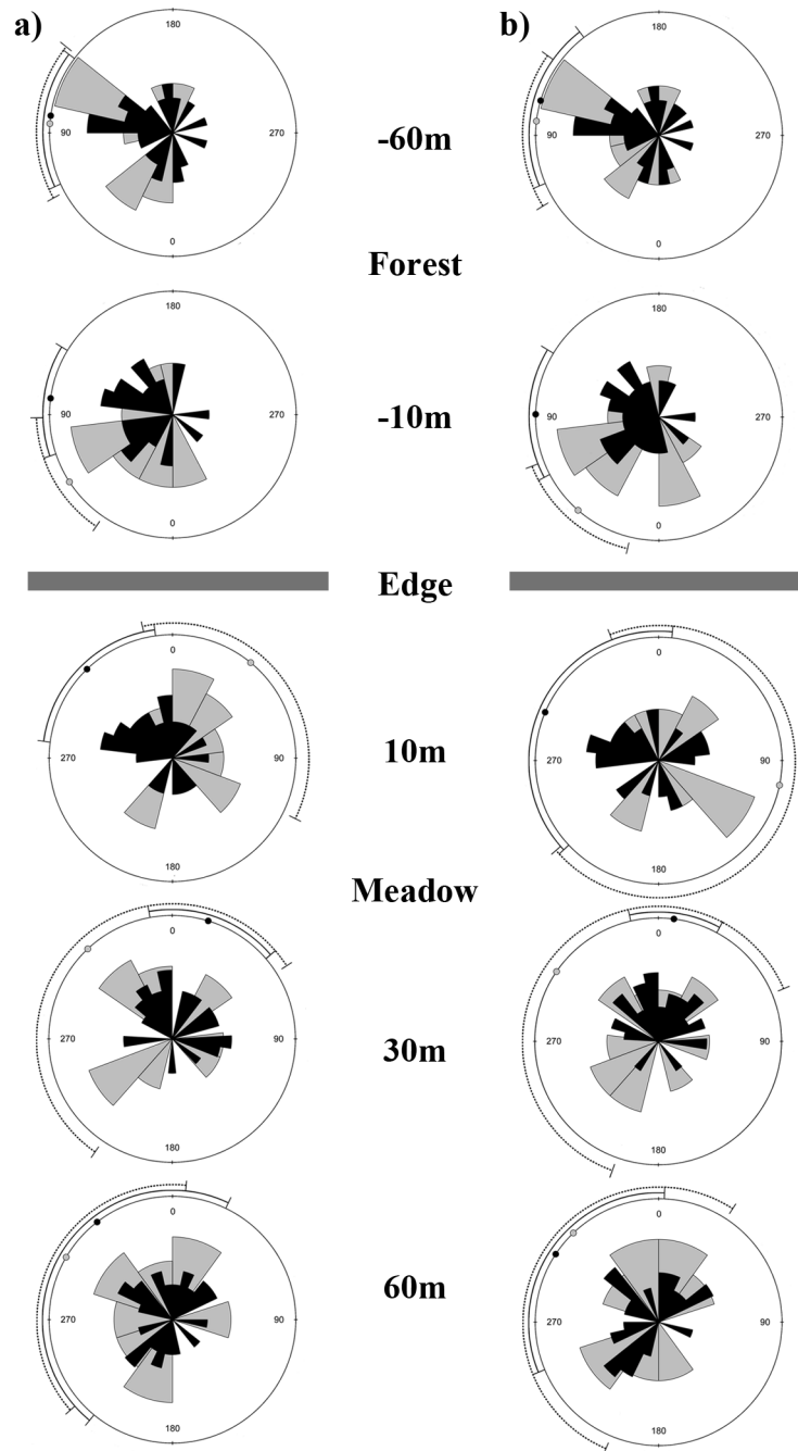
Figure 8. Rose diagrams show the distribution of (a) initial and (b) final divergence angles relative to the edge from all release points in the forest and in the meadow for P. troilus . Data were collected at three selected sites in Norfolk County during May-July 2012. Points on the circle are the mean directions bounded by parametric confidence intervals. Females are represented by gray and dotted lines, and black and solid lines represent males.
