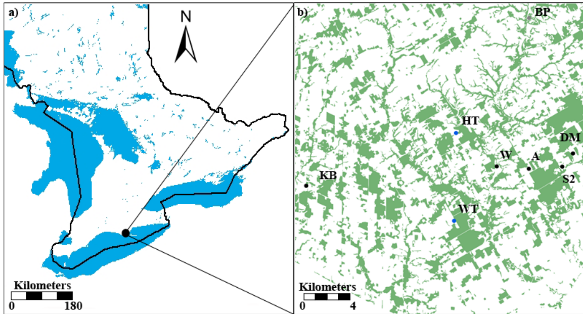
Figure 2. Map of Ontario and location of study in Norfolk County (a) and specific study sites (b) that were used to evaluate relative abundance in 2013 and conduct behaviour trials in 2012. Sites shown in blue were used for both surveying relative abundance and conducting flight behaviour trials, sites in black were used to survey abundance only, and sites in gray were used for behaviour trials only.
