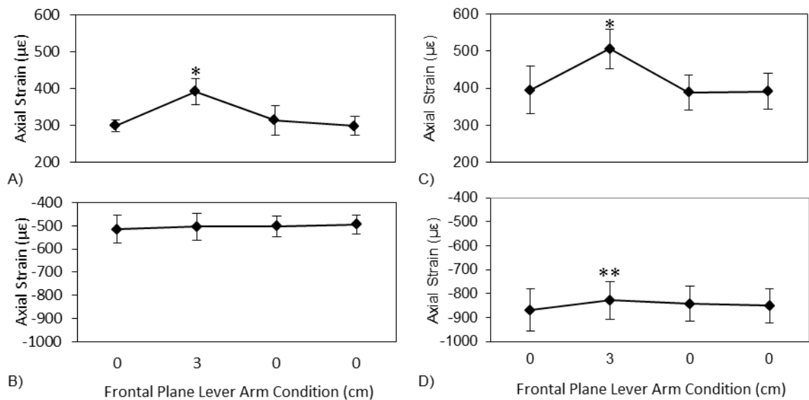
Figure 4.4: Means +/-SD for axial strain on the lateral cortical hinge (A & C) and on the medial opening wedge HTO plate (B & D) with a load of 900N (A & B) and 1400N (C & D) for each test condition.
