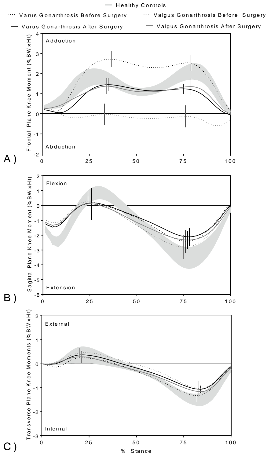
Figure 2.1: Ensemble averages ( n=13 ) of A) Frontal Plane B) Sagittal Plane and C) Transverse Plane knee moments plotted over 100% of stance. The shaded area represents the 95% confidence band for the healthy control population. Vertical bars represent 95% confidence intervals for peak values for both groups of patients before and after surgery.
