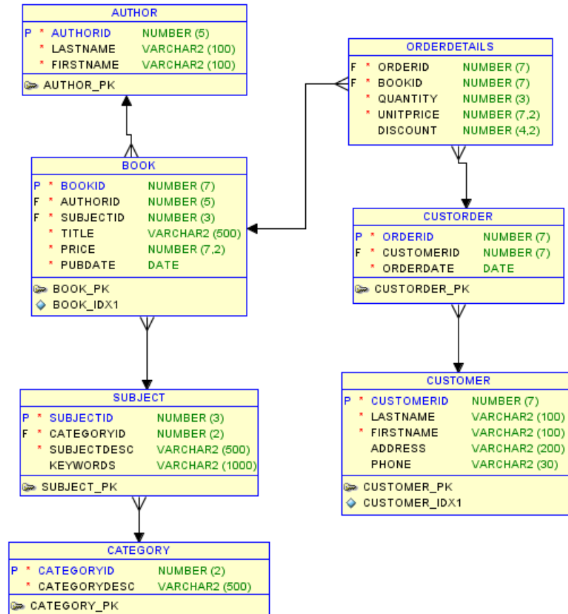
Figure 3: Database schema
