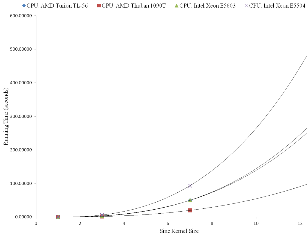
Figure 11: C implementation running time comparison across test beds.
