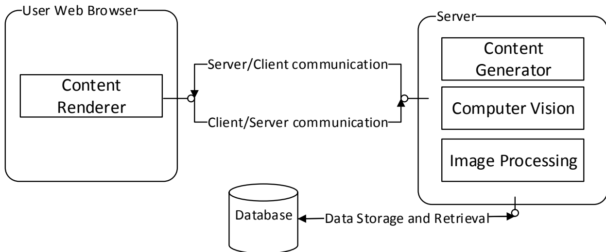
Figure 2-1: System architecture overview of SimCAM, showing the client (code deployed on the user's Web Browser), server and database component.
