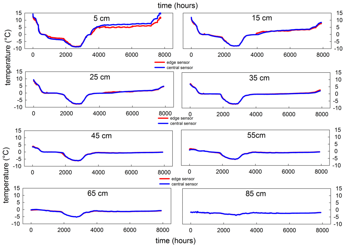
Figure 2-4. Temperature time series for all instrumented depths (5 to 85 cm) in the soil column. Depths of each time series are listed in each graph. Central and edge sensors nearly completely overlap each other and thus edge sensor cannot be seen for 45 cm and deeper.
