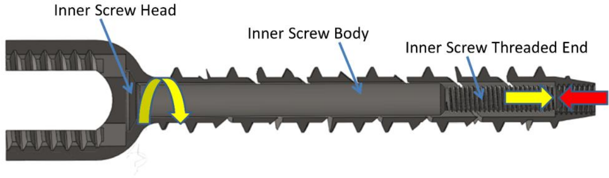
Figure B21: Section View of Helical Shell and Inner Screw at Initial Ingagement
