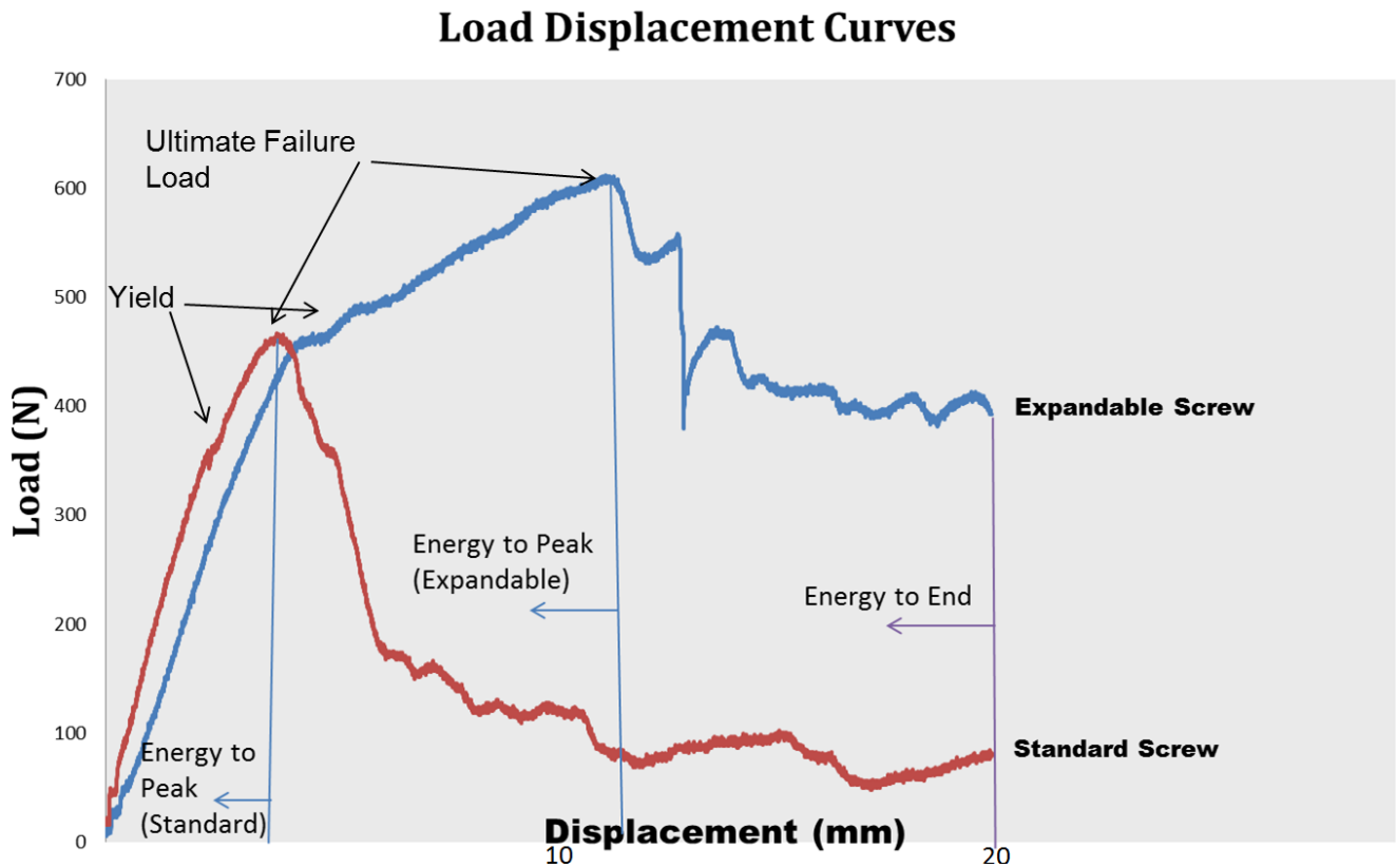
Figure 14: Sample Load Displacement Curve
