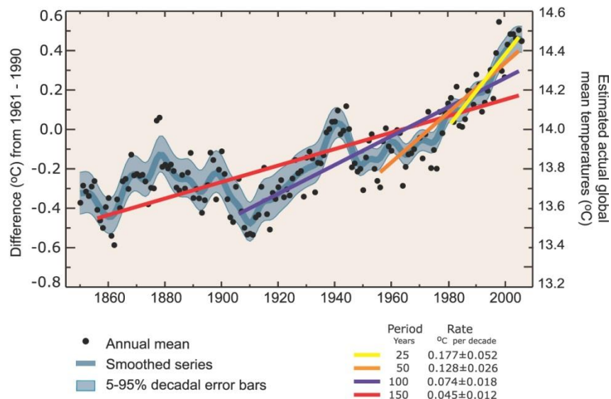
Figure 1: Global annual mean temperature for the duration 1856-2005 (plotted in black dots). Left hand axis shows temperature anomalies with respect to average temperatures recorded in the period 1961-1990 while right hand axis shows absolute temperature values (IPCC, 2007)
