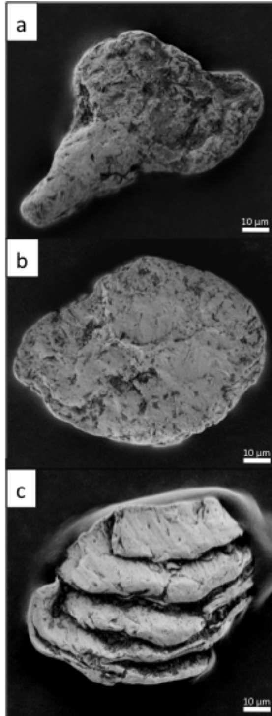
Figure 4.1. SEM characterisation of Rio Saldana gold grains. Low-magnification SEM micrographs of the three representative gold grain morphologies. Grains that appeared as semi-discoid ellipses had the greatest surface topography including irregular concave crevices and convex ridges (a). Discoid ellipse grains were flatter with smoother surfaces in comparison to the semi-discoid ellipse grains (b). Stacked discoid ellipses were composed of multiple grains of varying size (c).
