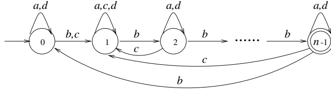
Figure 5.21: The DFA B used for showing that the upper bound in Theorem 5.22 is attainable when m \geq 2 and n, p \geq 1
