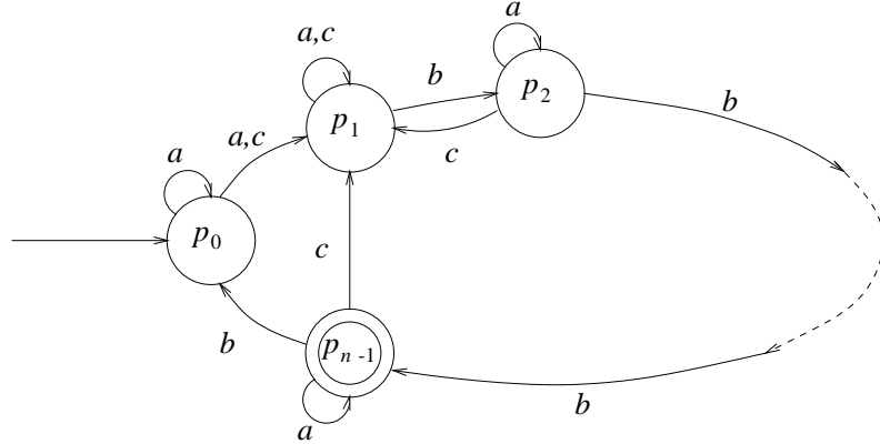
Figure 3.3: Witness DFA B for the second case of Theorem 3.1
