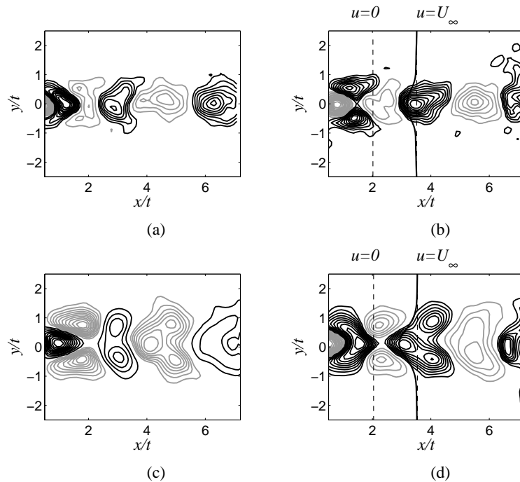
Figure 4.9. Modes 7 & 8 from POD of vorticity (positive - black, negative - grey) of: (a)-(b) circular- and (c)-(d) triangular-edged bodies. Time-averaged velocity profiles are shown for x=2t .
