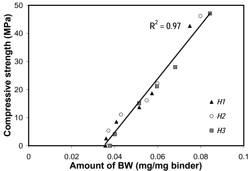
Figure 6-7: Relation between degree of hydration (amount of BW) and compressive strength development for the PHCM mixtures.
