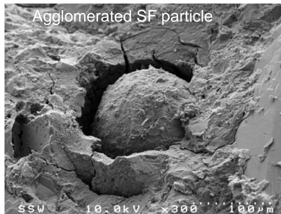
Figure 4-5: Scanning electron micrograph for agglomerated silica fume in SRA mixture with w/c=0.22 .
