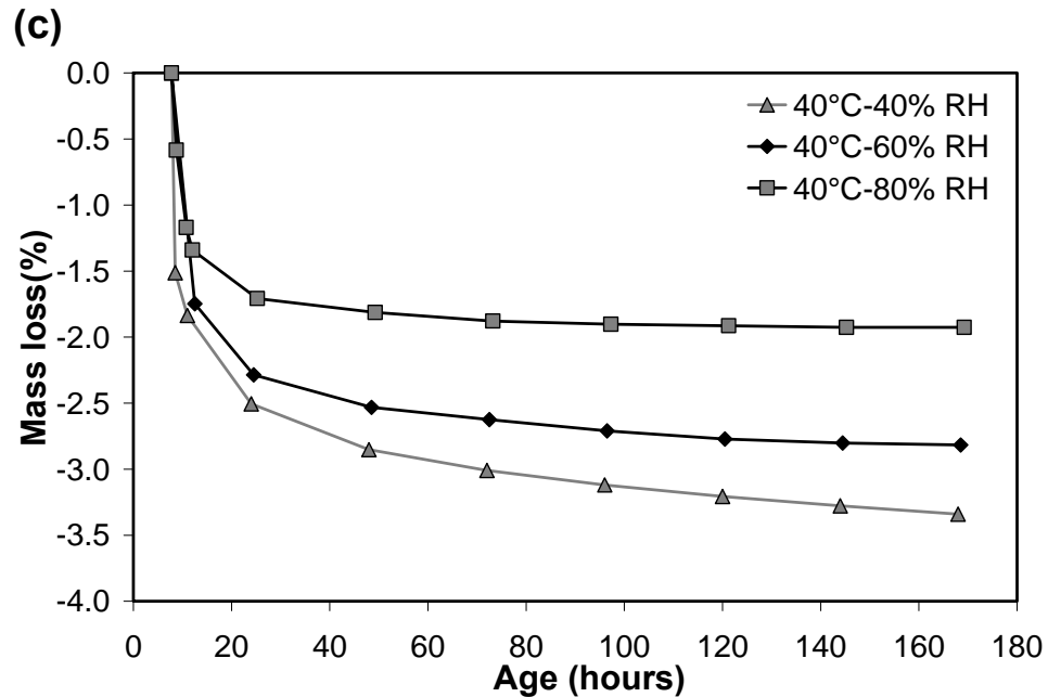
Figure 4-10 Cont'd: Change in mass loss Vs. ambient humidity for w/c=0.25 +2\% SRA mixture at a) 10^{\circ}\text{C} , b) 20^{\circ}\text{C} , and c) 40^{\circ}\text{C} .
