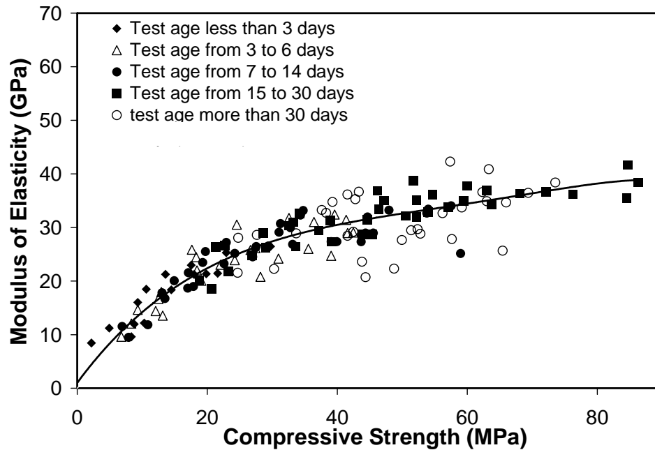
Figure 2-8: Modulus of elasticity to compressive strength ratio data classified by concrete age [after Zhao, 1990].
