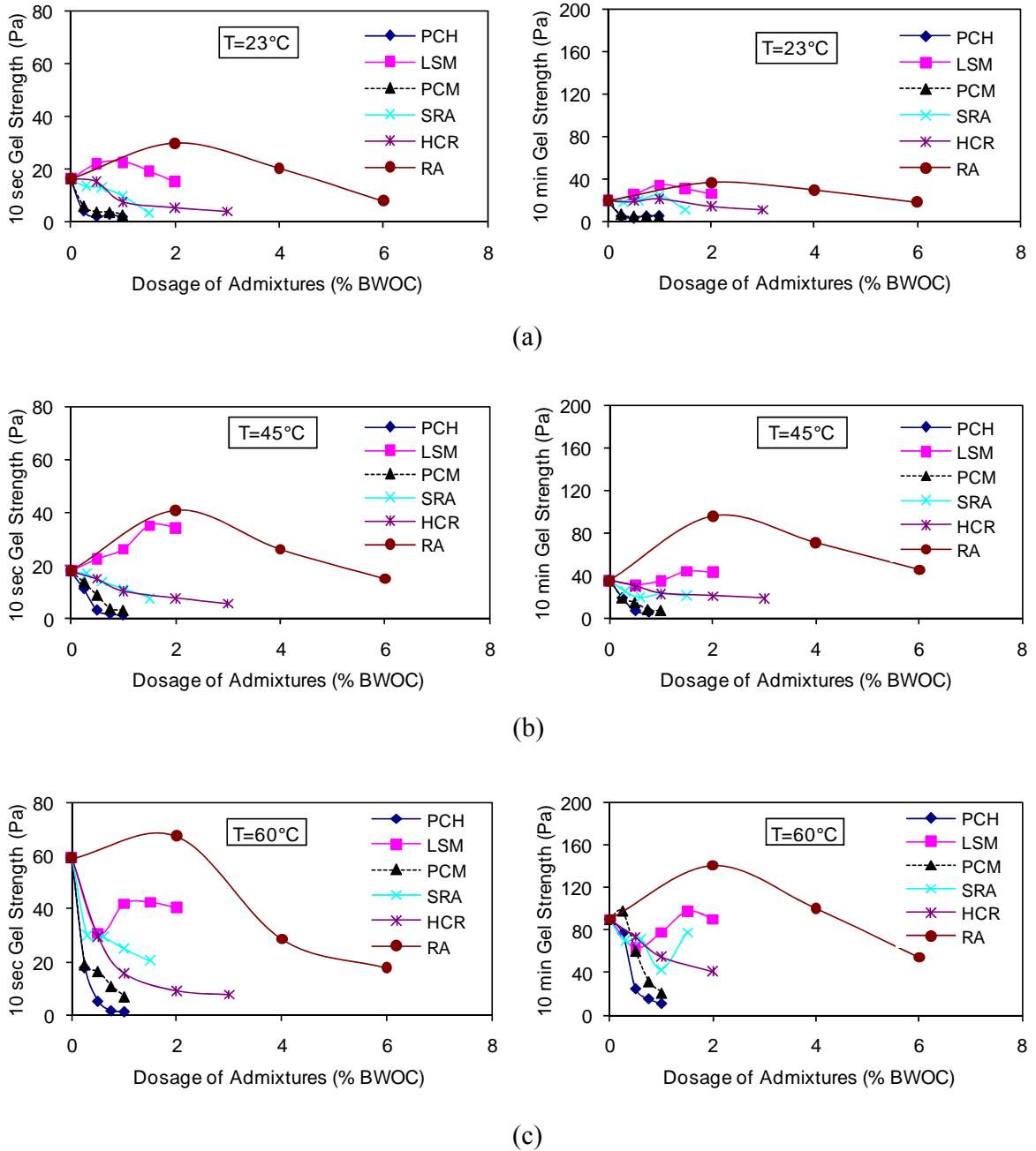
Figure 4.22 10-sec and 10-min gel strength of oil well cement slurries incorporating different admixtures at various temperatures, (a) T=23°C, (b) T=45°C, and (c) T=60°C (w/c = 0.44).
