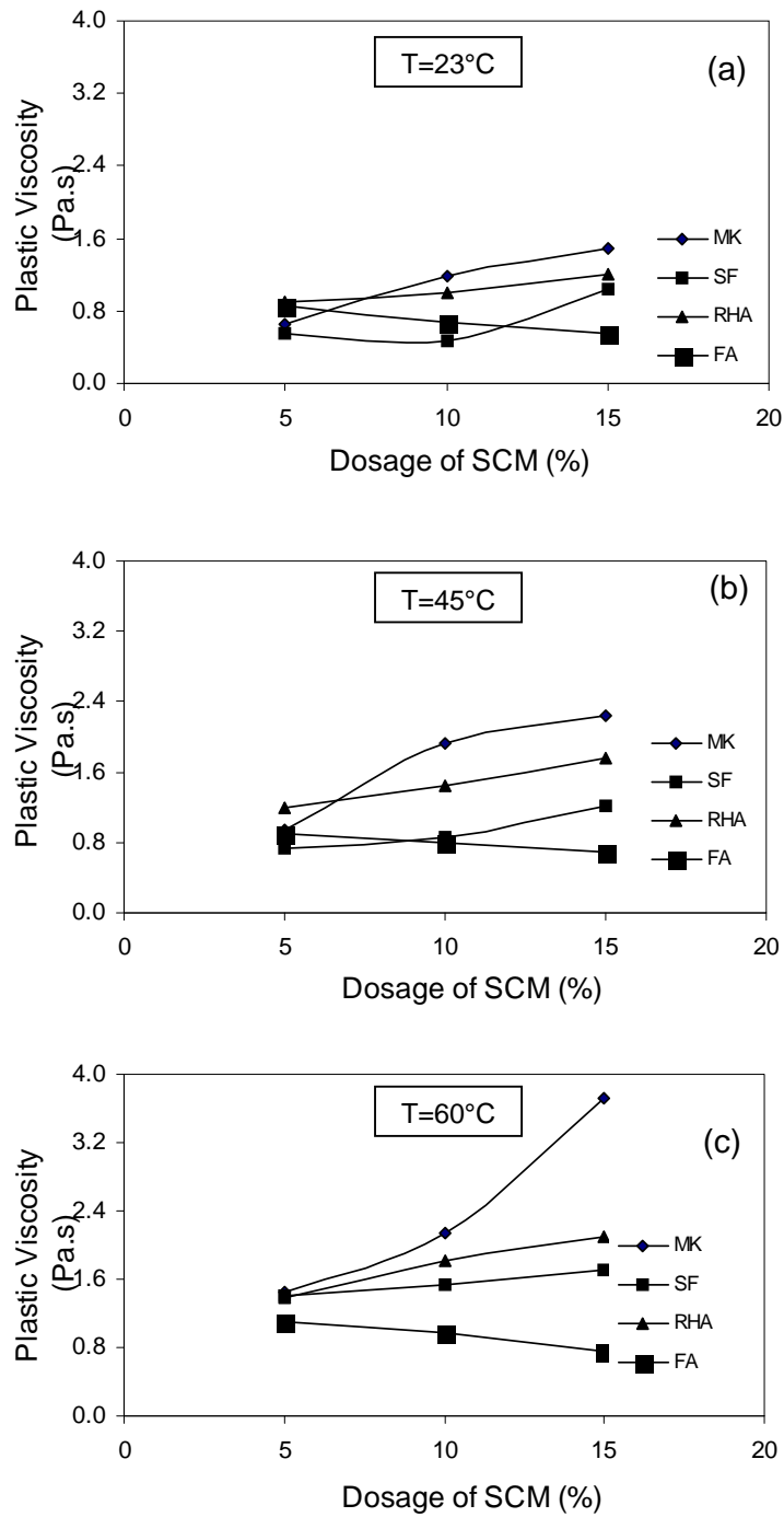
Figure 5.4 Variation of plastic viscosity of OWC slurries with type and dosage of SCM at (a) 23°C, (b) 45°C and (c) 60°C.
