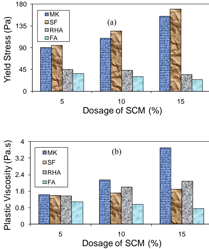
Figure 7.2 Variation of rheological properties of OWC slurries with type and dosage of SCM but without PCH at 60°C; (a) yield stress and (b) plastic viscosity.
