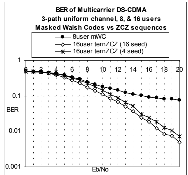
Fig. 4. BER comparison for different ternary sequences
