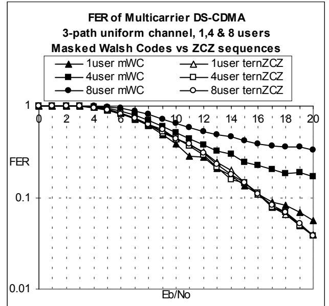
Fig. 3. FER Performances in a multipath Channel
