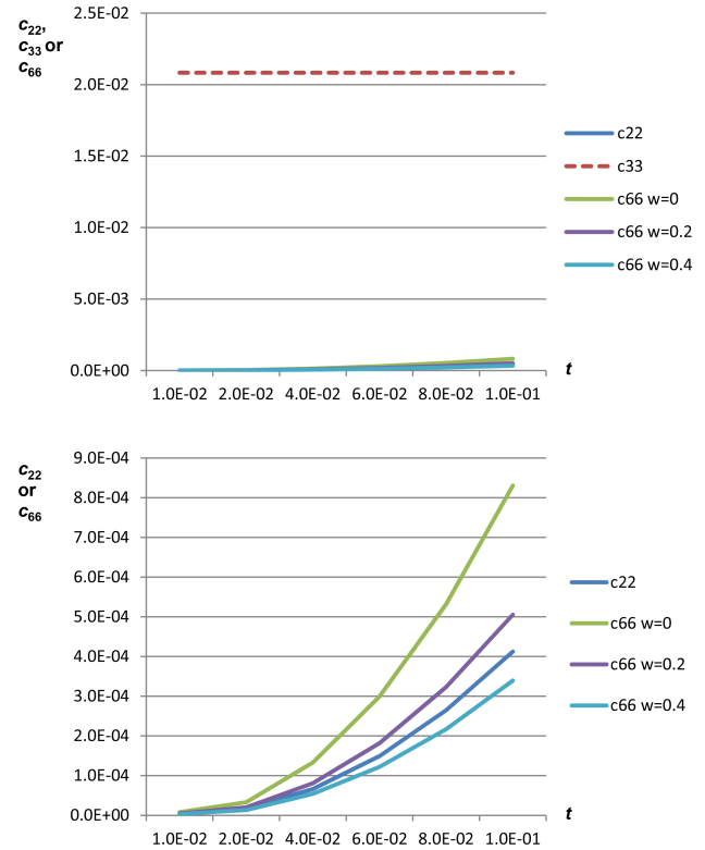
(a) Compliance affected by t
