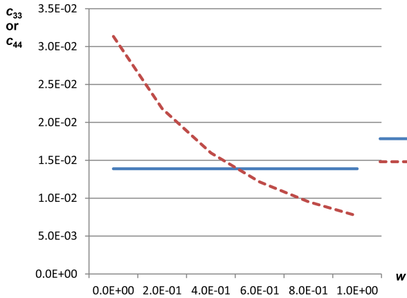
(b) Compliance affected by w
