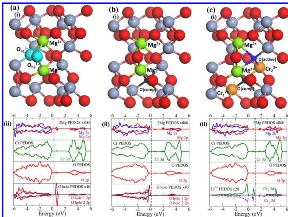
Figure 7: The local atomic structure and calculated PEDOS plots of 2Mg doped Cr 2 O 3 for (a) two Mg dopants, (b) charge compensated structure, and (c) active oxygen vacancy. The green, grey, red, light blue and orange spheres show the lattice positions of the Mg dopant, Cr cation, O anion, O atom with hole, and reduced Cr cations respectively. The small black and blue sphere shows the location of the compensated and active oxygen vacancies. For the PEDOS plots, the blue, red and green lines show the s, p and d state contributions to the VB and CB. The top of the VB is aligned to 0eV, and the dashed black line shows the position of the Fermi level.
