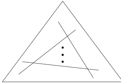
( n ) lines in \mathbb{P}^2
