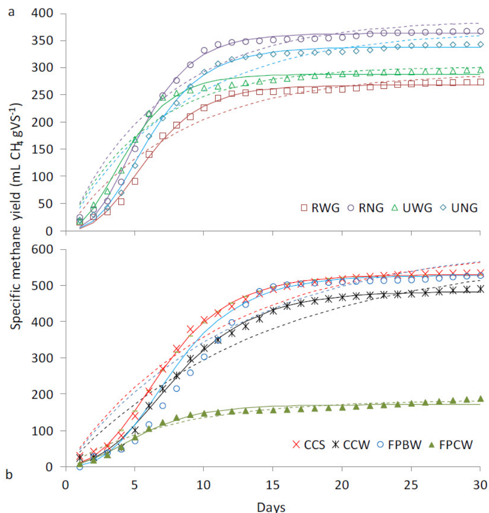
Figure 3 BMP cumulative methane yields for (a) household samples and (b) commercial & processing samples
