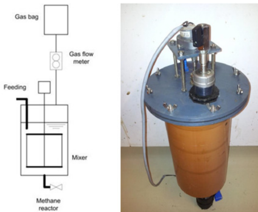
Figure 2 Continuously stirred tank reactor (5L) used for semi continuous trial
