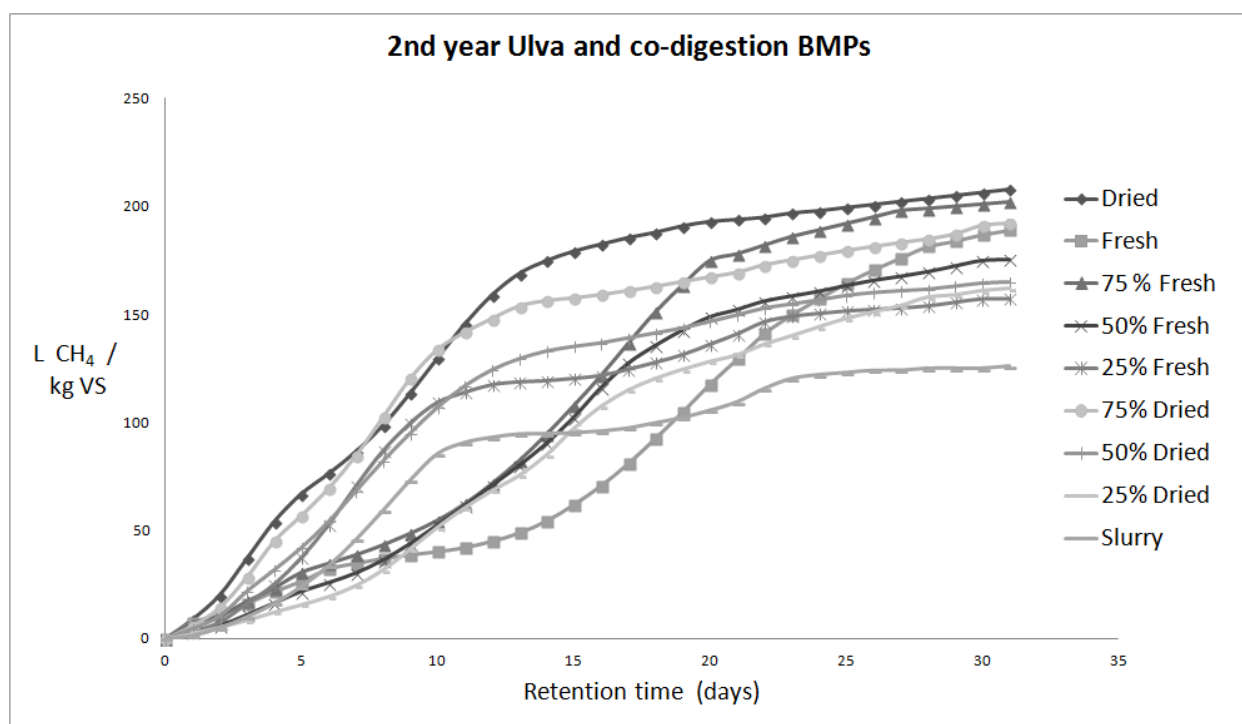
Figure 6.5 Cumulative BMP for U. lactuca from the second year in mono and co-digestion.
