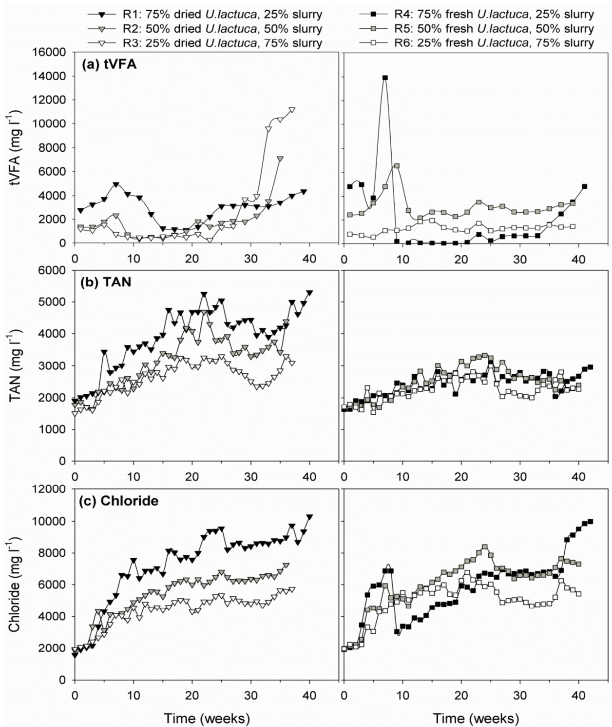
Figure 7.2 Environmental parameters R1 – R6.
