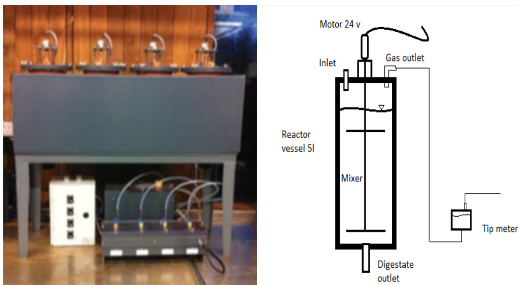
Figure 4.1 Semi-continuous digestion system consisting of 5L reactors and tipping bucket measuring device.
