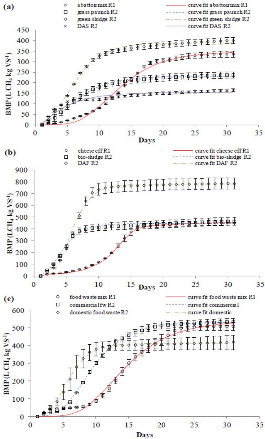
Figure 3 (a) BMP of abattoir waste round 1 & 2 (b) BMP of cheese processing waste round 1 & 2 (c) BMP of food waste round 1 & 2
