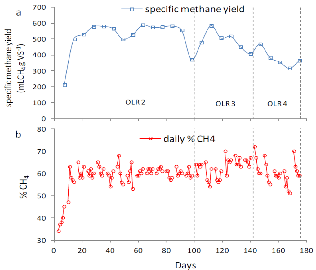
Figure 4 (a) Weekly average specific methane yield and (b) daily methane percentage
