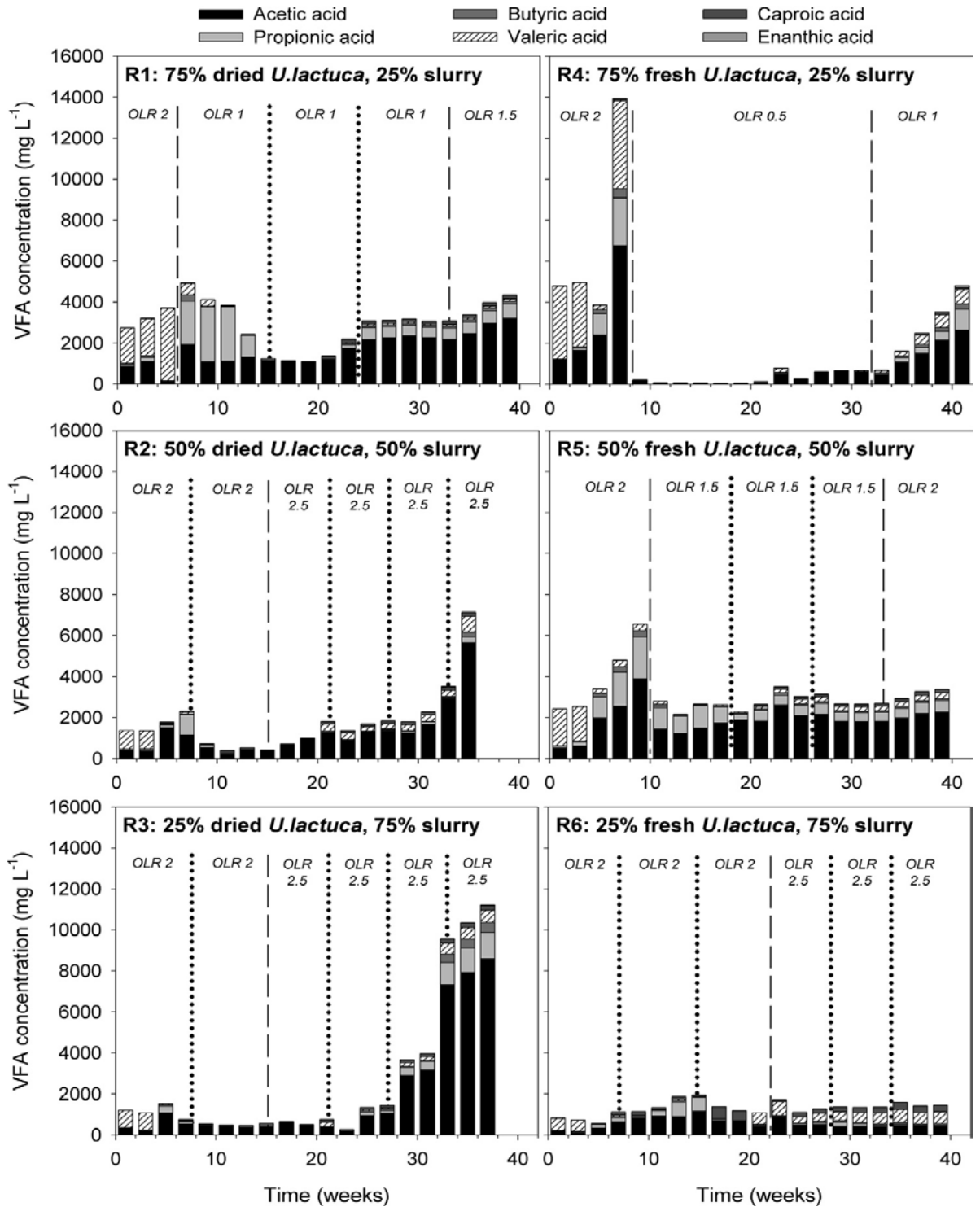
Figure 7.3 Breakdown of VFA concentrations for reactors R1-R6
