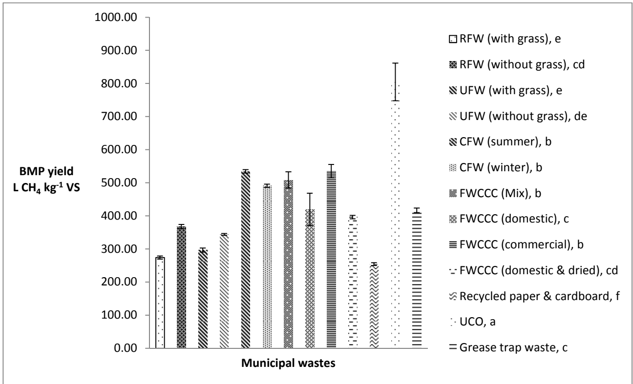
Figure S3.5 Statistical analysis of municipal wastes and BMP assay results.
