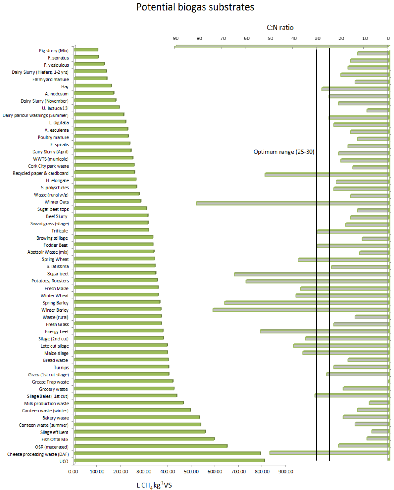
Figure S3.7 Comparison between a selection of BMP yields and C:N ratios.
