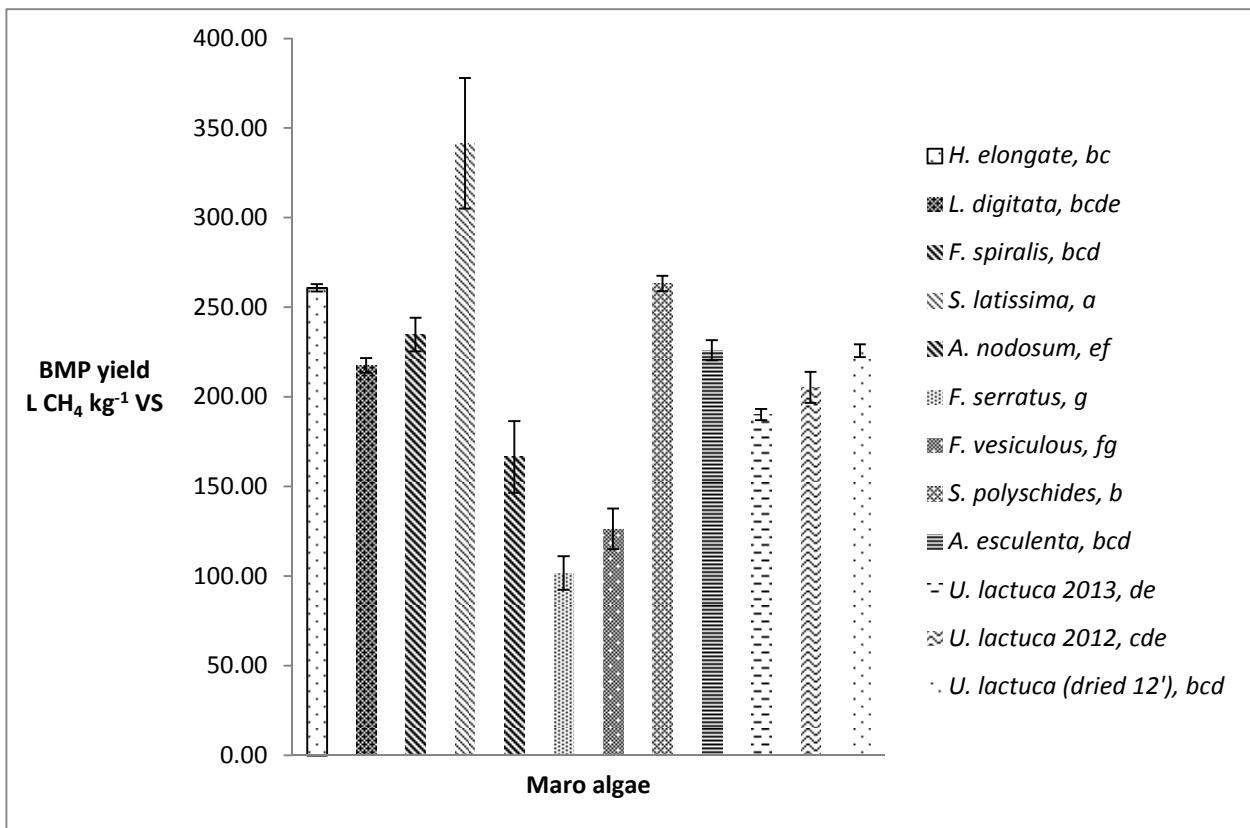
Figure S3.6 Statistical analysis of macro algae and BMP assay results.
