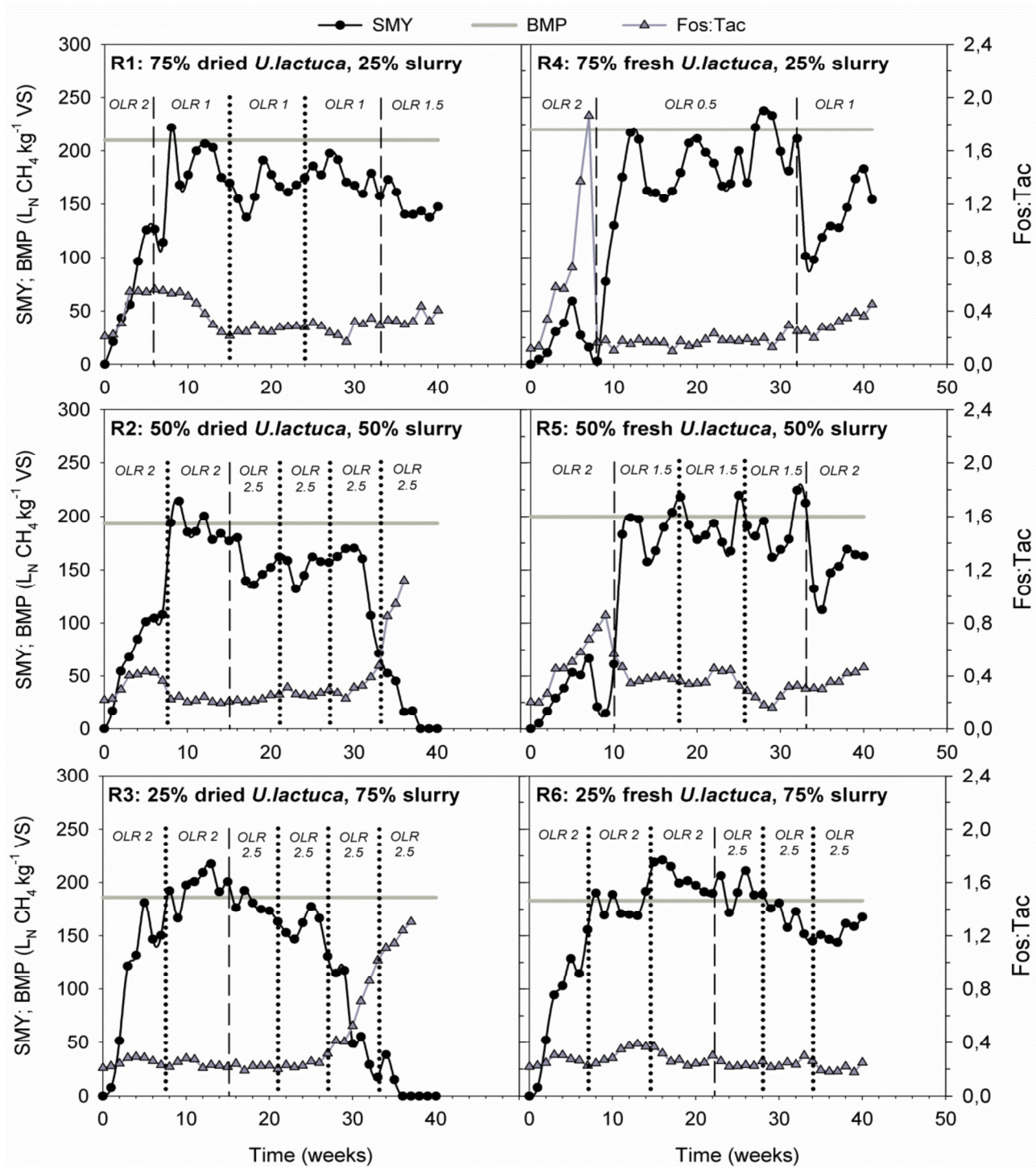
Figure 7.1 Performance and operational parameter curves R1 – R6.
