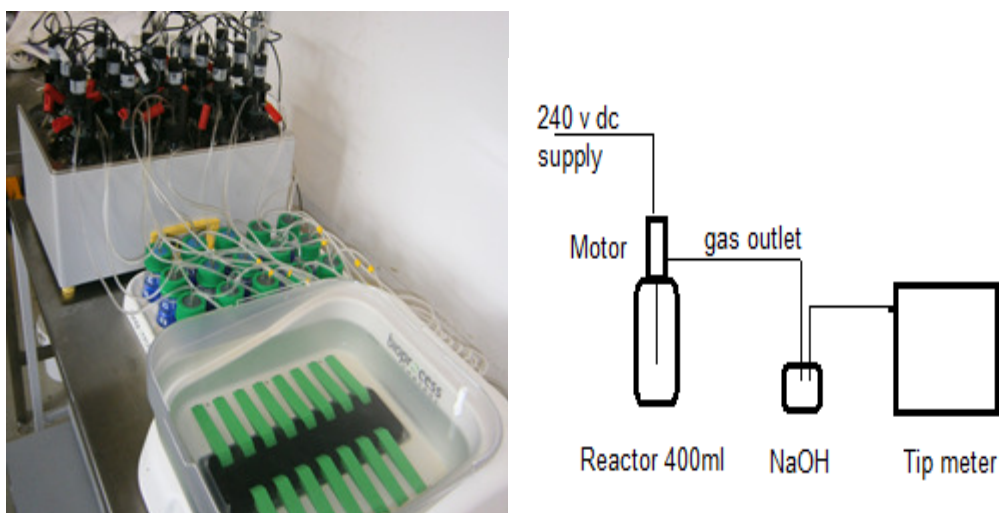
Figure 6.3 Biomethane potential test system.
