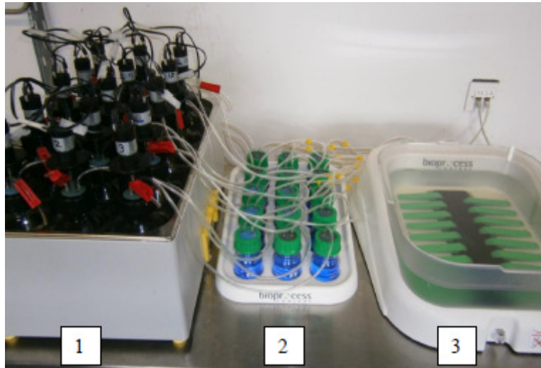
Figure 2 BMP apparatus used in the paper: Automatic Methane Potential Test System II (Bioprocess Control Sweden AB). 1. Water bath with 15 No. 500 ml bottle reactors: 2. Carbon dioxide fixing unit: 3. Gas flow measuring unit
