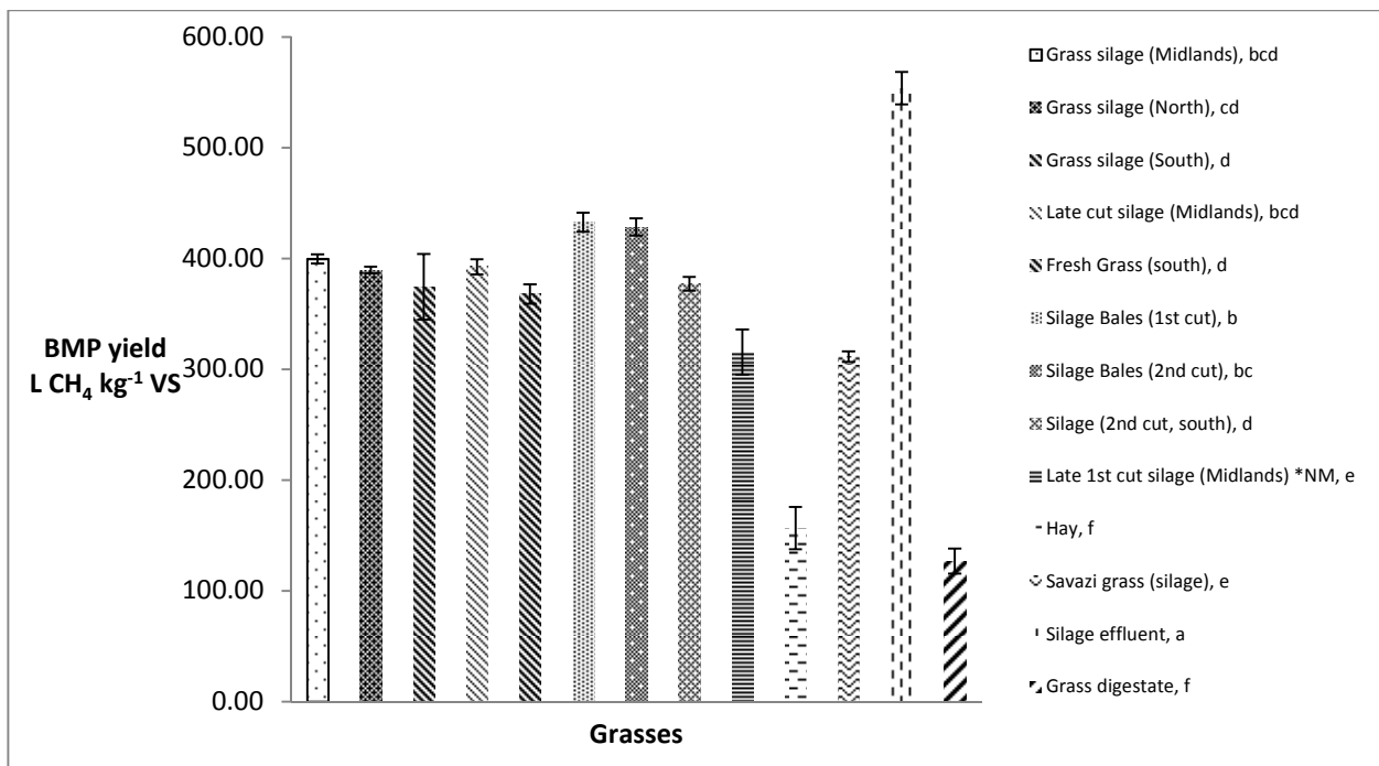
Figure S3.2 Statistical analysis of grass substrates and BMP assay results.
