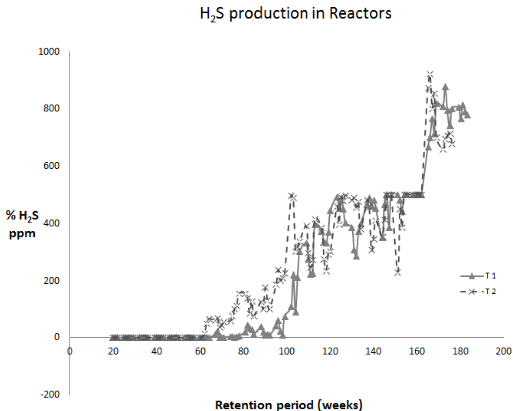
Figure 4.3 Levels of H 2 S (ppm) in biogas from T1 and T2.
