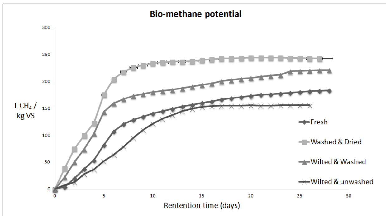
Figure 6.4 Cumulative BMP, fresh and pre-treated samples from Year 1.
