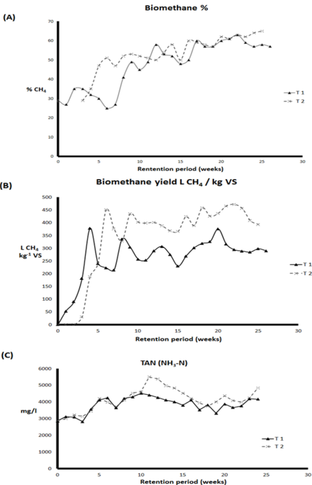
Figure 4.2 Biomethane yields and TAN concentrations for T1 and T2.
