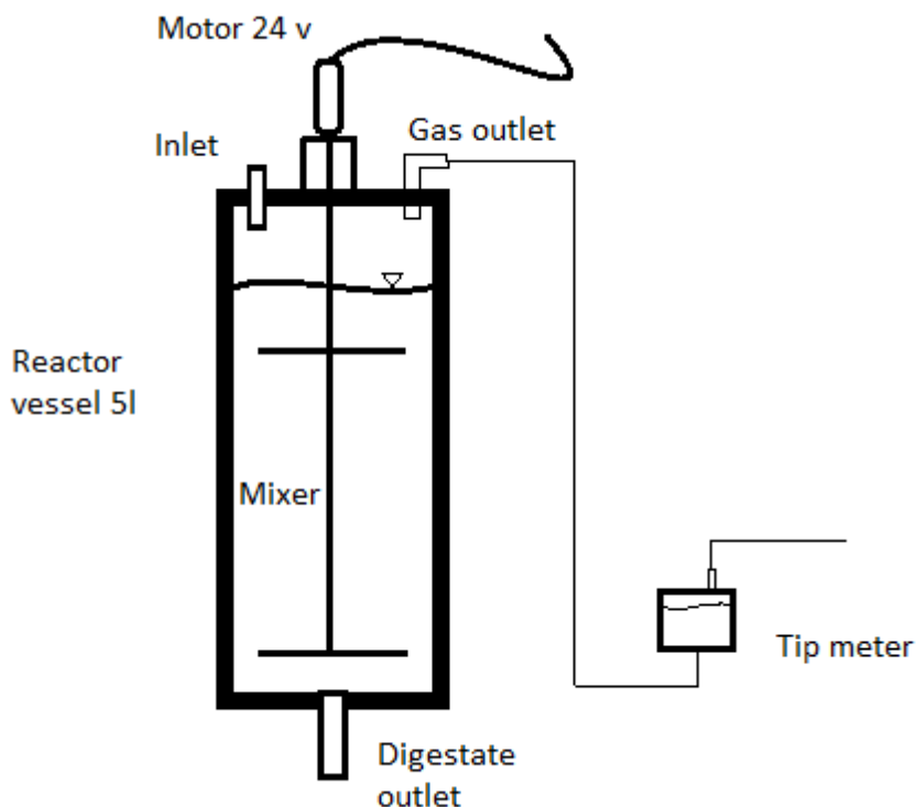
Figure 1. Schematic of Reactor set up for R1 and R6.
