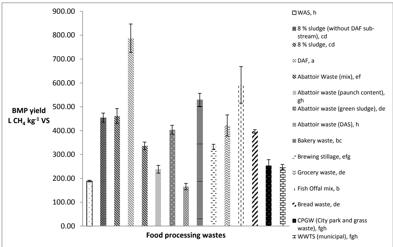
Figure S3.4 Statistical analysis of food processing wastes and BMP assay results.
