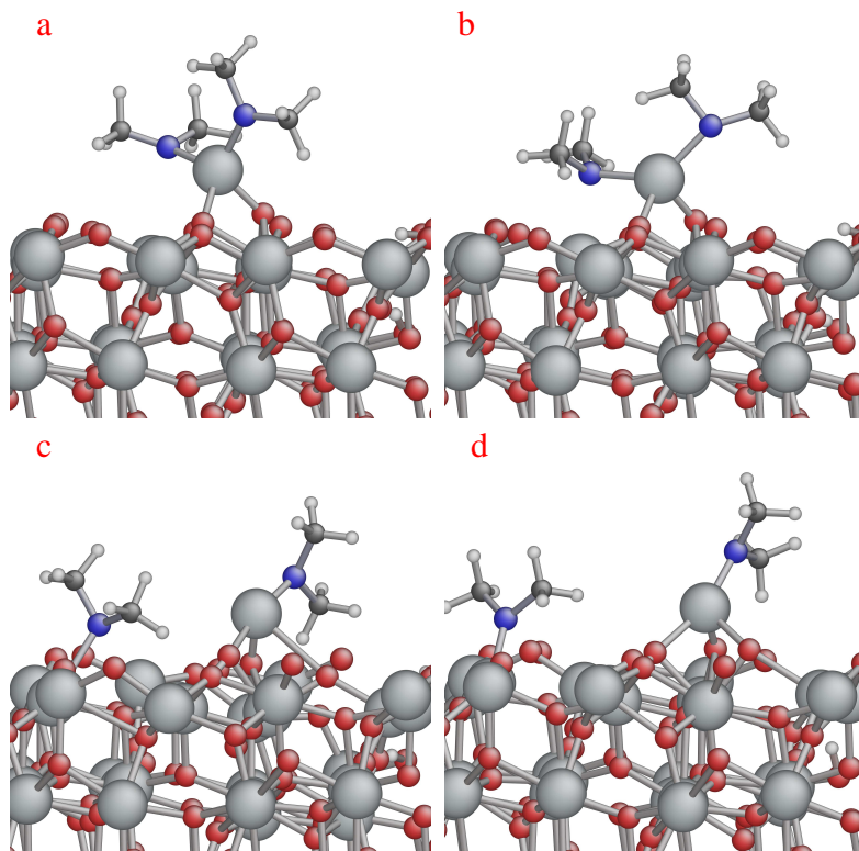
Figure 9: The amide group of the densified HfX 2 was transferred to under-coordinated hafnium at the surface; snapshots are from ab initio MD calculation, starting at T = 500 K and running for 0.4 ps.
