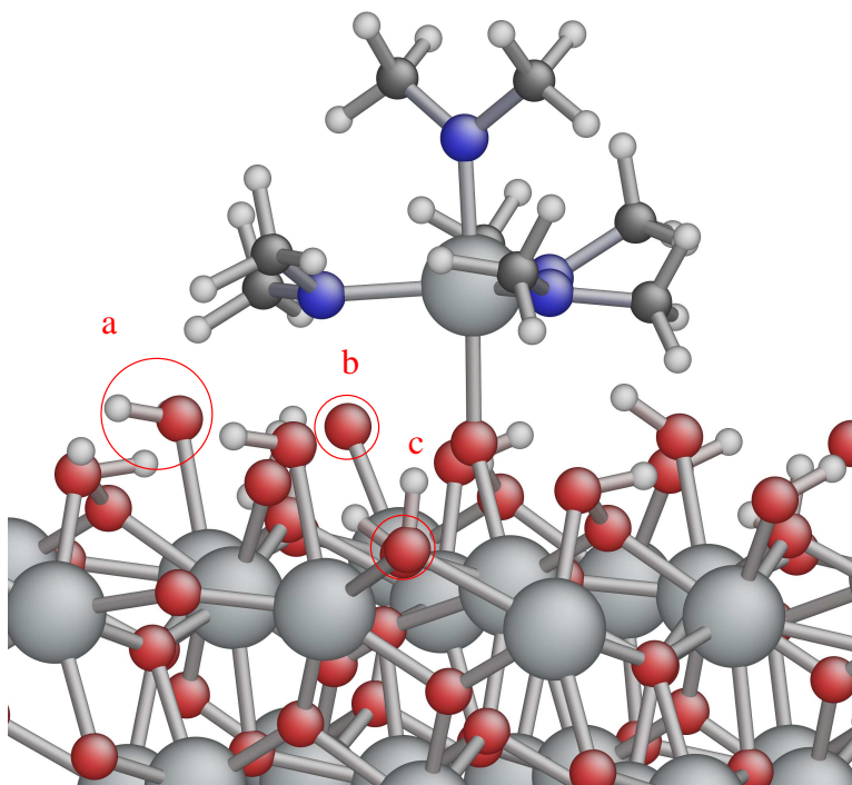
Figure 1: Optimized geometry for adsorption of HfX 4 molecule onto OH terminated HfO 2 . Terminal hydroxyl group (a), terminal oxygen (b) and bridging oxygen (c) are highlighted. The HfX 4 is anchored to a terminal oxygen. (Red = O, Blue = N, White = H, large grey = Hf, small grey = C).
