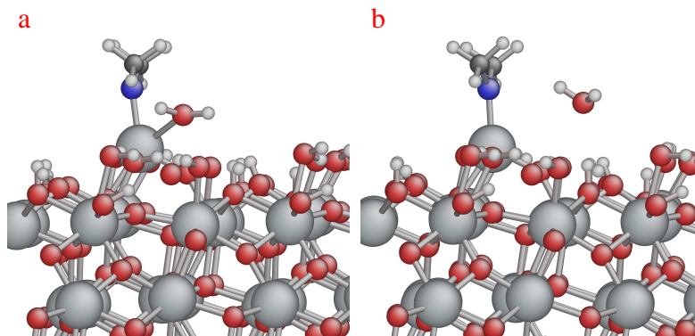
Figure 10: The H 2 O molecule is not dissociated when there are not enough Lewis acid and base sites in terms of number; snapshots are from optimization.
