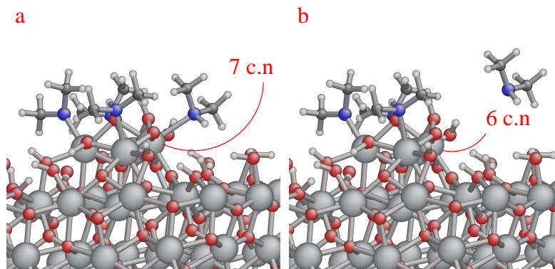
Figure 12: Dissociation of HX from seven coordinated hafnium during water pulse. Four oxygen (originally adsorbed as H 2 O) are coordinated to the cluster and dissociation of HX from the resulting 7-coordinate Hf is more favourable than the situation in Figure 11.
