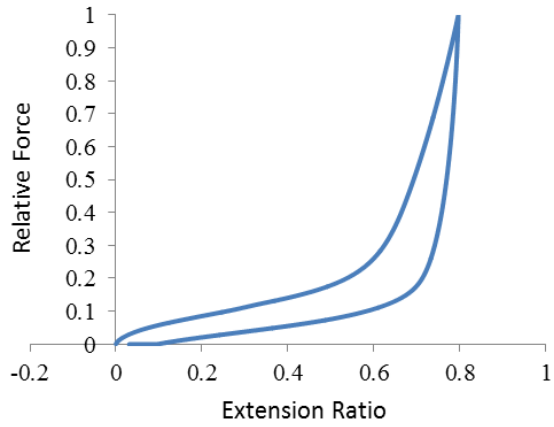
Figure 3. Seaflex elastic component Force – extension curve
