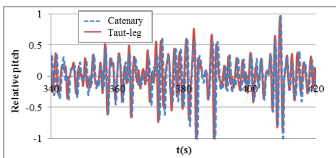
Figure 9. Pitch motion (normalised by the maximal significant height of pitch motion)
