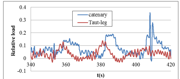
Figure 10. Loads on front anchor (normalised by the largest load on anchors)
