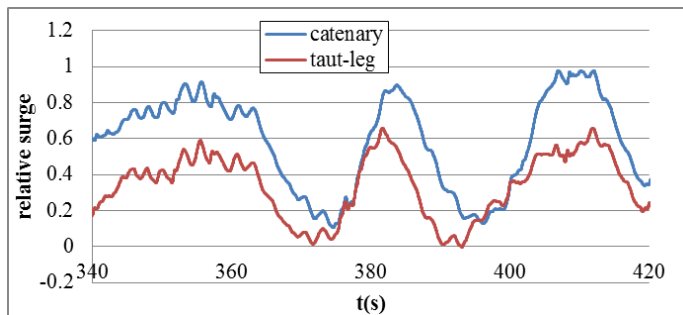
Figure 7. Surge motion (normalised by using the largest excursion)
