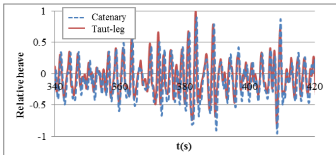
Figure 8. Heave motion (normalised by the maximal significant height of heave motion)
