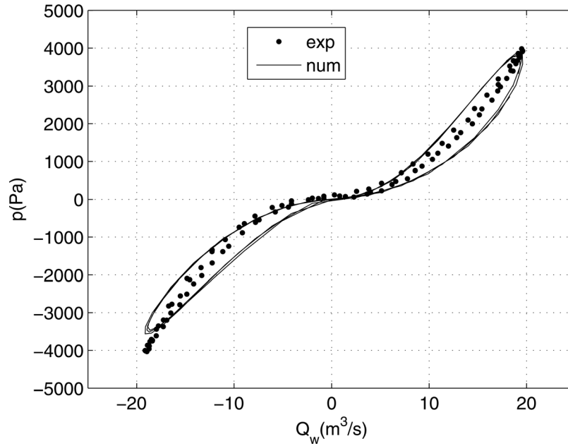
FIG. 11. Chamber pressure, p , and flowrate, Q_w ( \epsilon = 50 ).
