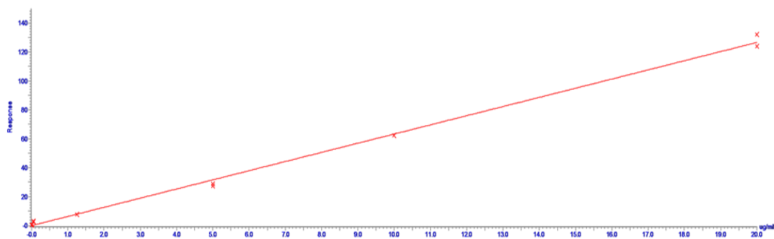
Fig. 1. MVAL standard curve (20µg/ml-3.125ng/ml) with R 2 of the line equal to 0.997725
