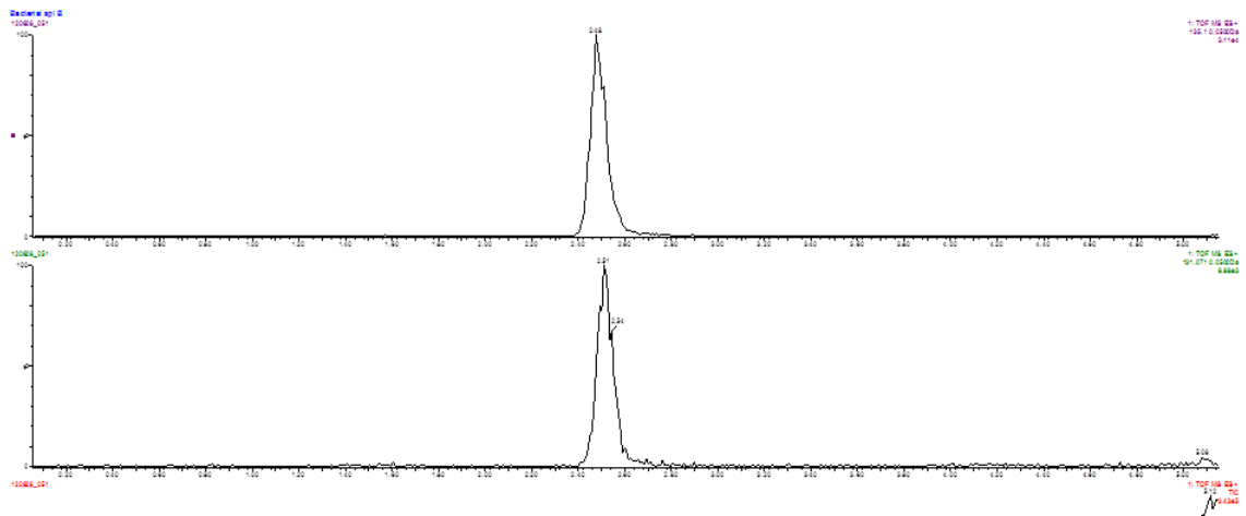
Fig.2. Chromatogram peaks for analyte MVAL (above) and internal standard D4-MVAL (below)
