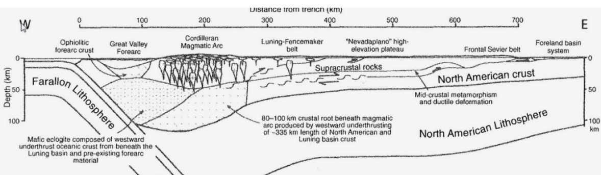
Figure 4. 4 Typical cross section across the Cordillera (From Hildebrand, 2009).
