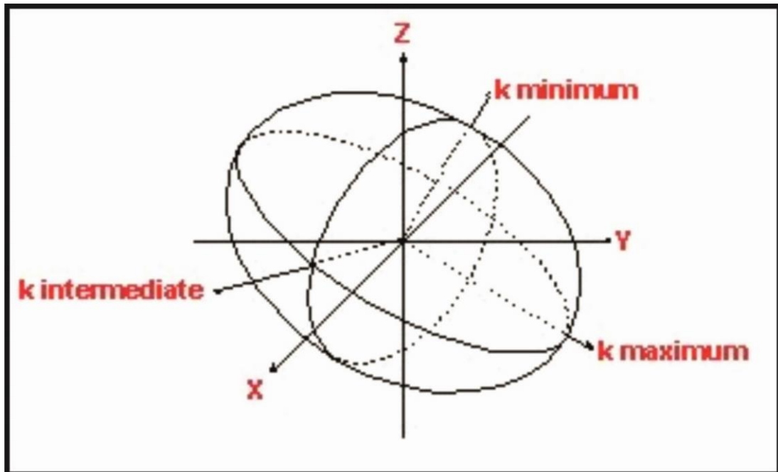
Figure 3. 2 Magnetic susceptibility ellipsoid with three mutually orthogonal axes. These axes correspond to the maximum (K1), intermediate (K2) and minimum (K3) susceptibility values, whose magnitudes and orientations can be defined in Cartesian coordinates.
