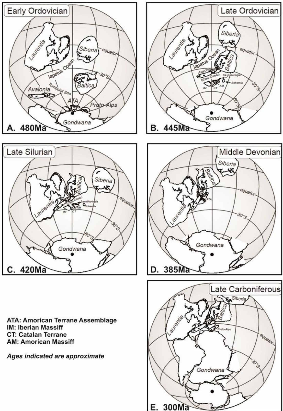
Figure 6. 2 Palaeogeographic reconstructions from Early Ordovician to Late Carboniferous (from Schaez, 2004), detailing the Caledonian Orogeny (A--C), the Acadian Orogeny (D) and the onset of the Variscan Orogeny (E).
