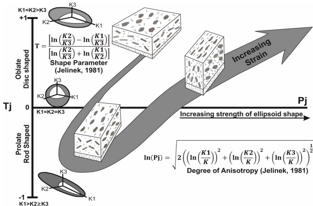
Figure 3. 11 The progression in ellipsoid shapes under progressive deformation using a Pj-Tj plot. Pj represents degree of anisotropy and increases in this imply increasing strength of the ellipsoid shape. Tj represents the shape parameter; positive numbers imply an oblate ellipsoid, whereas negative values imply a prolate ellipsoid, perfectly triaxial ellipsoids are represented by Tj values of 0. Modified from Pares (2004). The representative fabric block diagrams are from Ramsay and Huber (1983).
