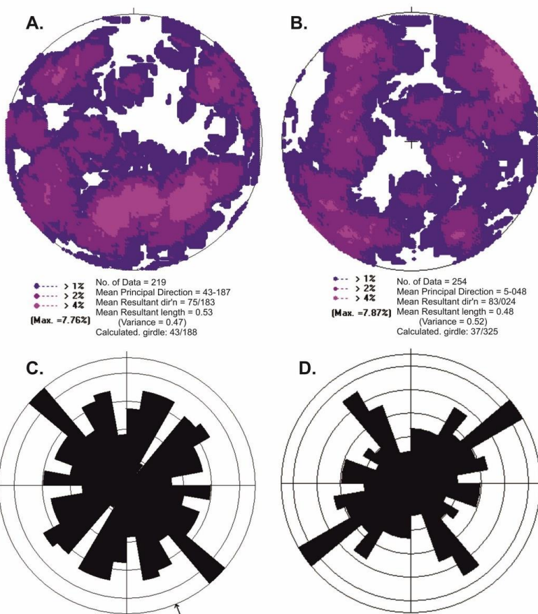
Figure 4. 28 Contoured stereonets and rose diagrams of K1 from the data in Figure 4.26. Contoured plot of K1 of paramagnetic specimens. B. Contoured plot of K1 of diamagnetic specimens. C. Rose diagram of K1 for paramagnetic specimens. D. Rose diagram of K1 for diamagnetic specimens.
