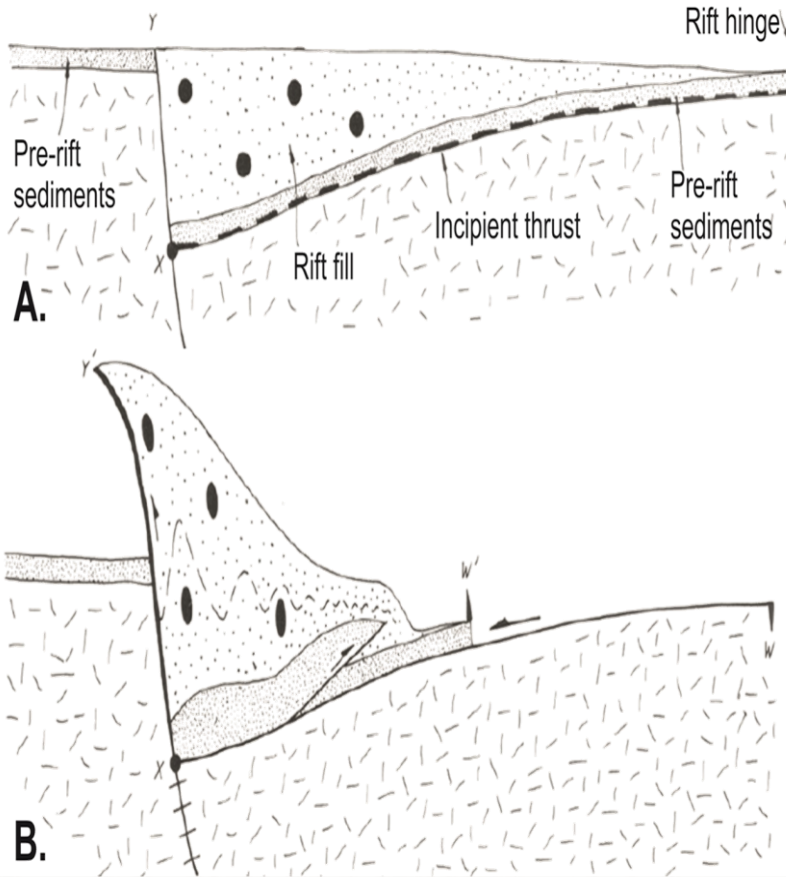
Figure 6. 16 Buttrressing structures in a reactivation setting (from Butler, 1989). A. Pre-deformation rift structures. B. Post-deformation structures, with decollement shown between the basement and cover material. In this model the zone of highest deformation is shown nearest to the buttressing surface, additionally there is no reactivation of the original normal fault.
