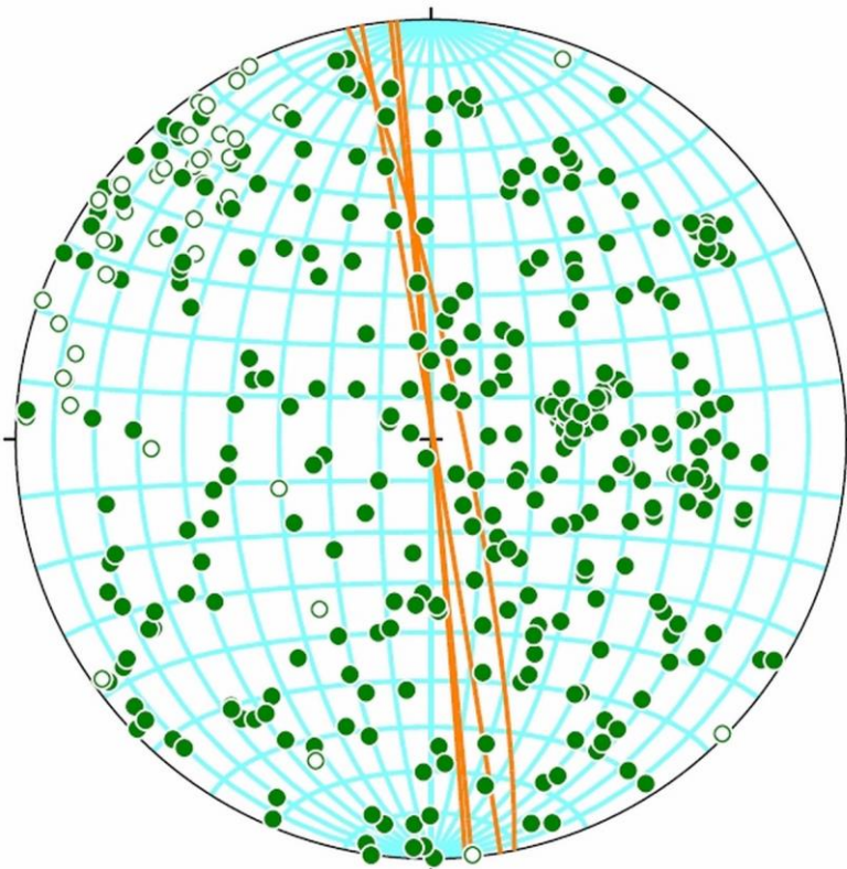
Figure 5. 20 Stereographic projections of minimum susceptibility axes (K3) for all specimens with correction for bedding. Bedding is now horizontal. Typical cleavage planes are indicated in orange.
