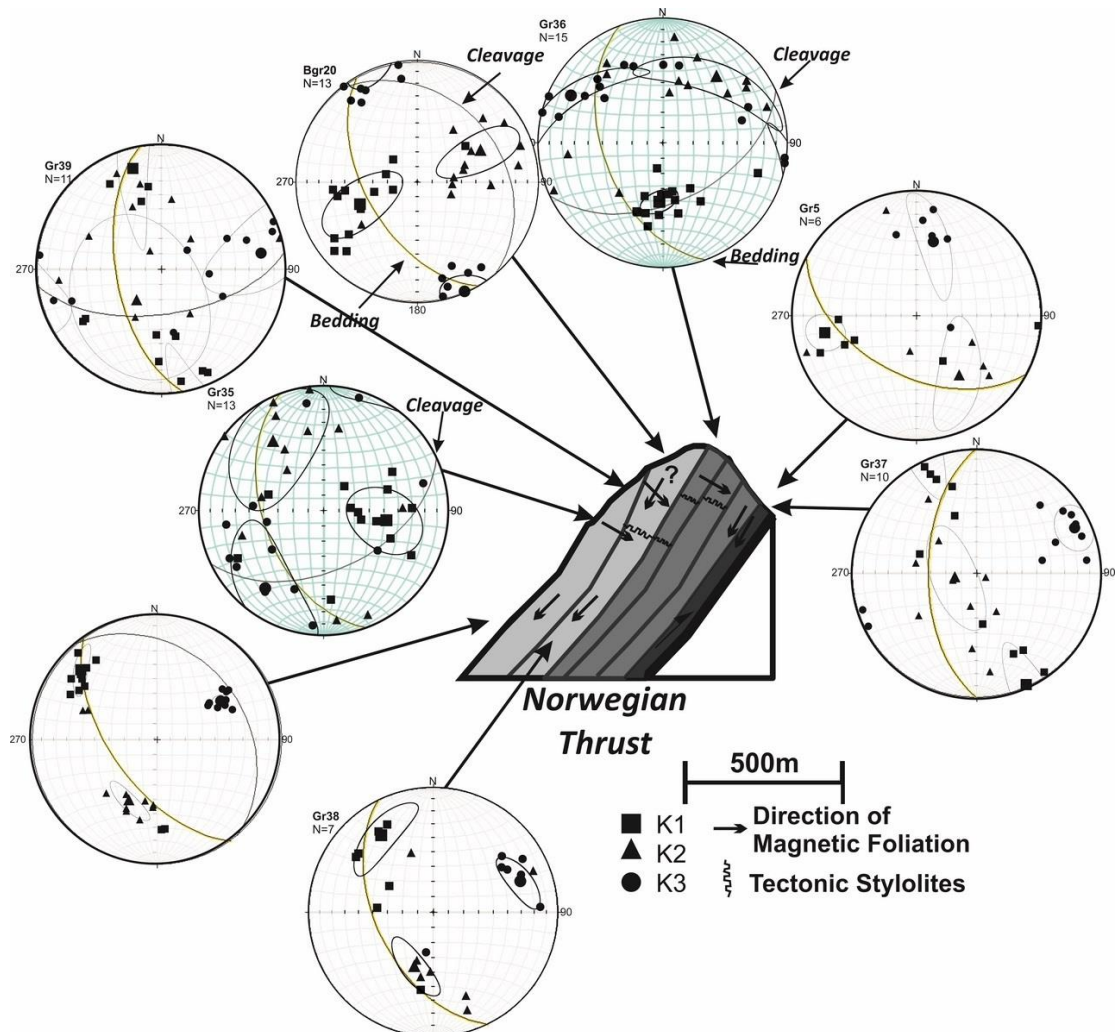
Figure 4. 34 Stereographic projections of principal susceptibility axes for block samples across the Norwegian thrust sheet. Also shown is the inclination of magnetic foliation relative to bedding and tectonic stylolites.
