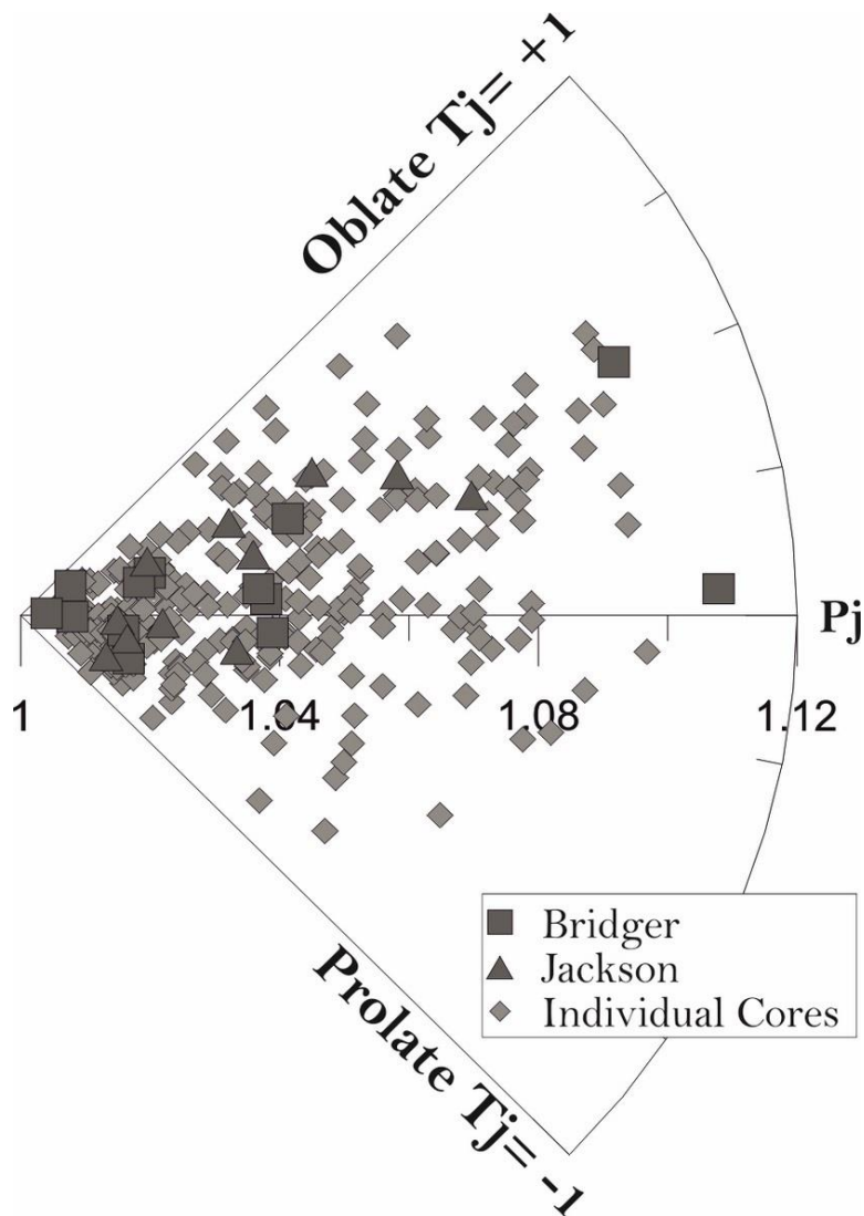
Figure 5. 11 Borradaile-Jackson Polar plot of all individual specimens as well as mean samples. This plot is similar to T_j - P_j plot in that it displays the same information, with the advantage that samples with weaker anisotropies ( P_j ) plotting closer to the origin regardless of shape.
