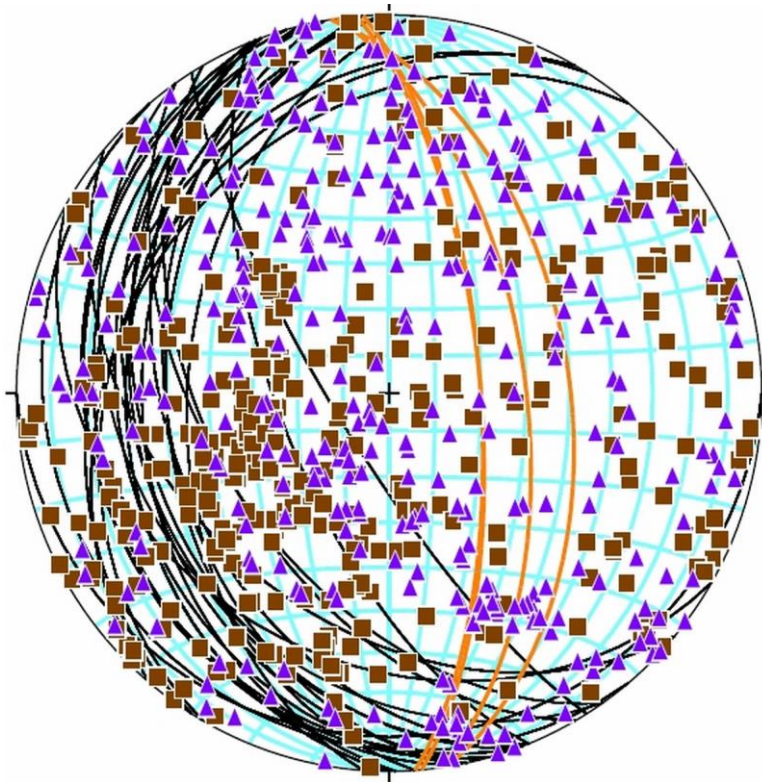
Figure 5. 17 Stereographic projections of maximum and intermediate susceptibility axes (K1 & K2) for all specimens. Individual bedding planes are plotted in black and primarily dip shallowly westward. Typical cleavage planes are plotted in orange.
