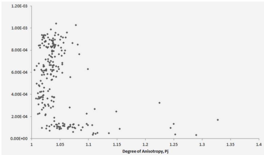
Figure 6. 39 Plot of degree of anisotropy versus susceptibiliy for individual specimens. There is no clear relationship between anisotropy and susceptibility.
