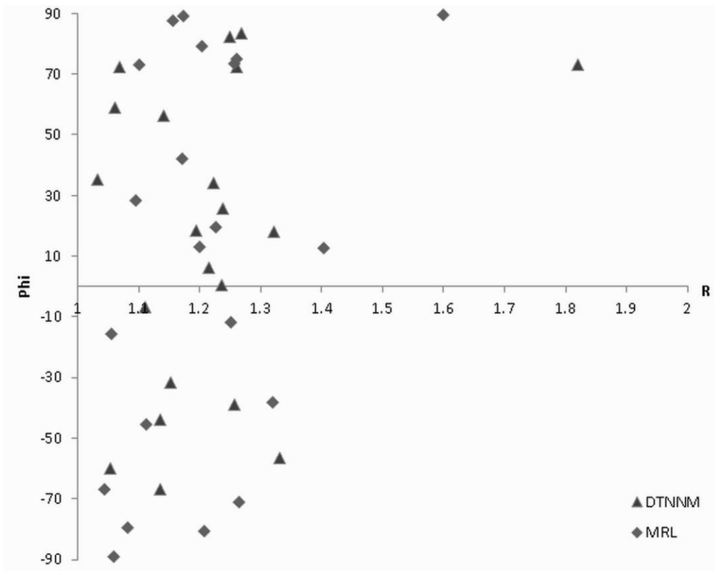
Figure 6.102 R/Phi for the C sections, in this case Phi orientations represent deviations away from the trace of bedding in the section.
