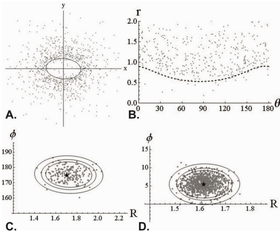
Figure 6.55 Strain estimates for Wb1A from the DTNNM and MRL analyses. A. Fry plot of the nearest neighbour data. B. Polar plot of the nearest neighbour data. C. DTNNM strain estimate and bootstrap data. D. MRL strain estimate and bootstrap data.
