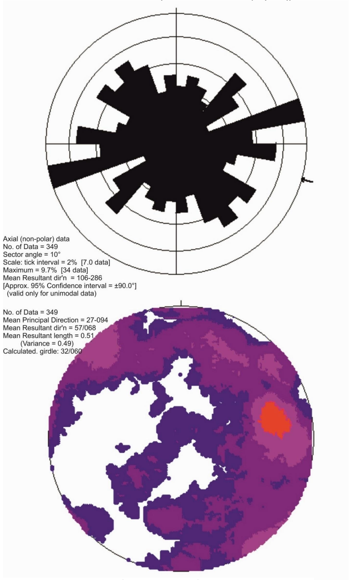
Figure 5. 14 Top: Rose diagram of the K3 orientations for all specimens. Bottom: Contoured plot of K3 plunge and trend.
