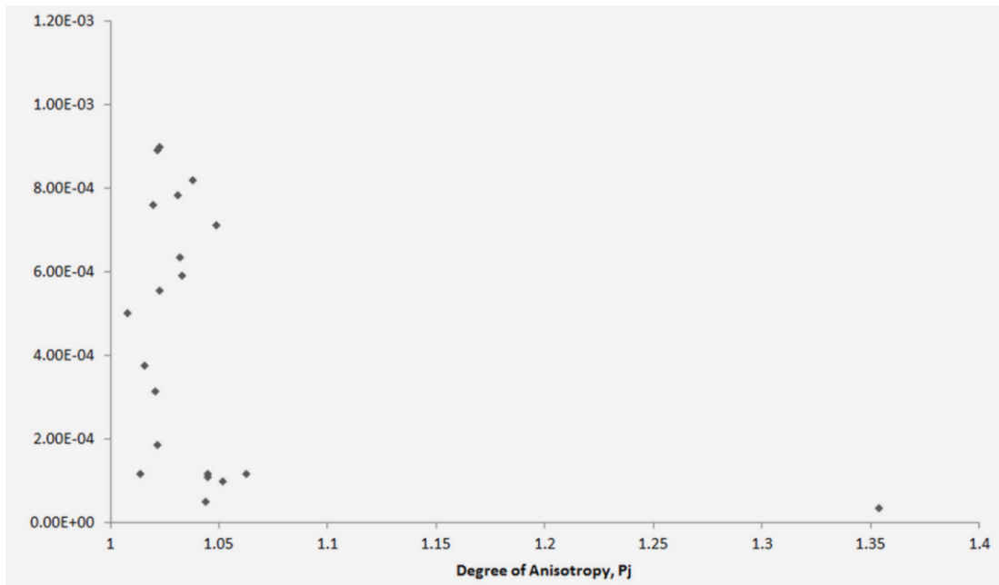
Figure 6. 40 Plot of degree of anisotropy versus susceptibiliy for samples. Again there is no clear relationship between anisotropy and susceptibility.
