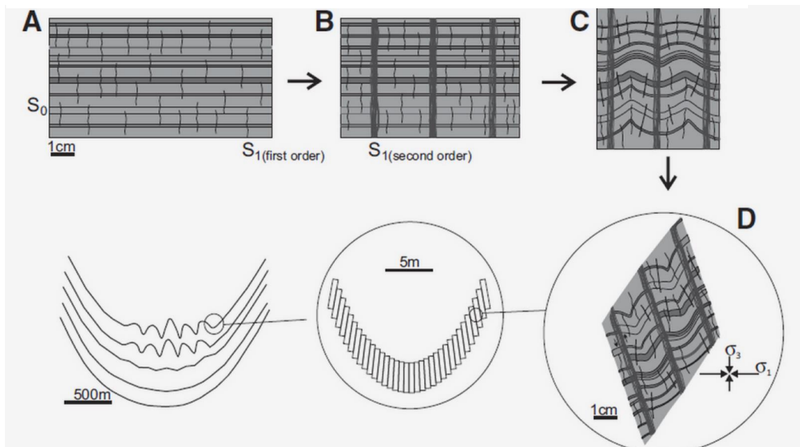
Figure 6. 23 Sheared cleavage development in the South Munster Basin, from Meere et al. (2013). A Initial cleavage development. B. Development of cleavage domains. C. Buckling and compressional faulting of cleavage domains. D. Regional and outcrop scale folding, leading to reverse simple shear along cleavage planes.
