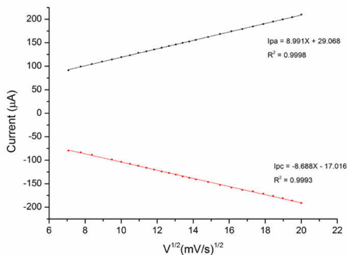
Figure 4.16: Cyclic voltammogram and the plot of the redox peak currents versus square root of the scan rate obtained at the SPE/Pd in 5 mM [\text{Fe}(\text{CN})_6]^{3-/4-} in 0.1M KCl solution at scan rate 50 to 400 mV/s.
