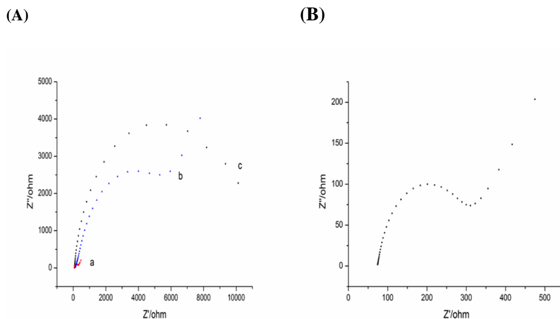
Figure 4.27: (A) Nyquist plots of [\text{Fe}(\text{CN})_6]^{3-/4-} in 0.1 M KCl solution with (a) a SPE, (b) a SPE/CM, and (c) a SPE/CM/Au. The frequency range is from 1 Hz to 100 kHz. (B) Nyquist plot of [\text{Fe}(\text{CN})_6]^{3-/4-} in 0.1 M KCl solution with a SPE/CM/Au.
