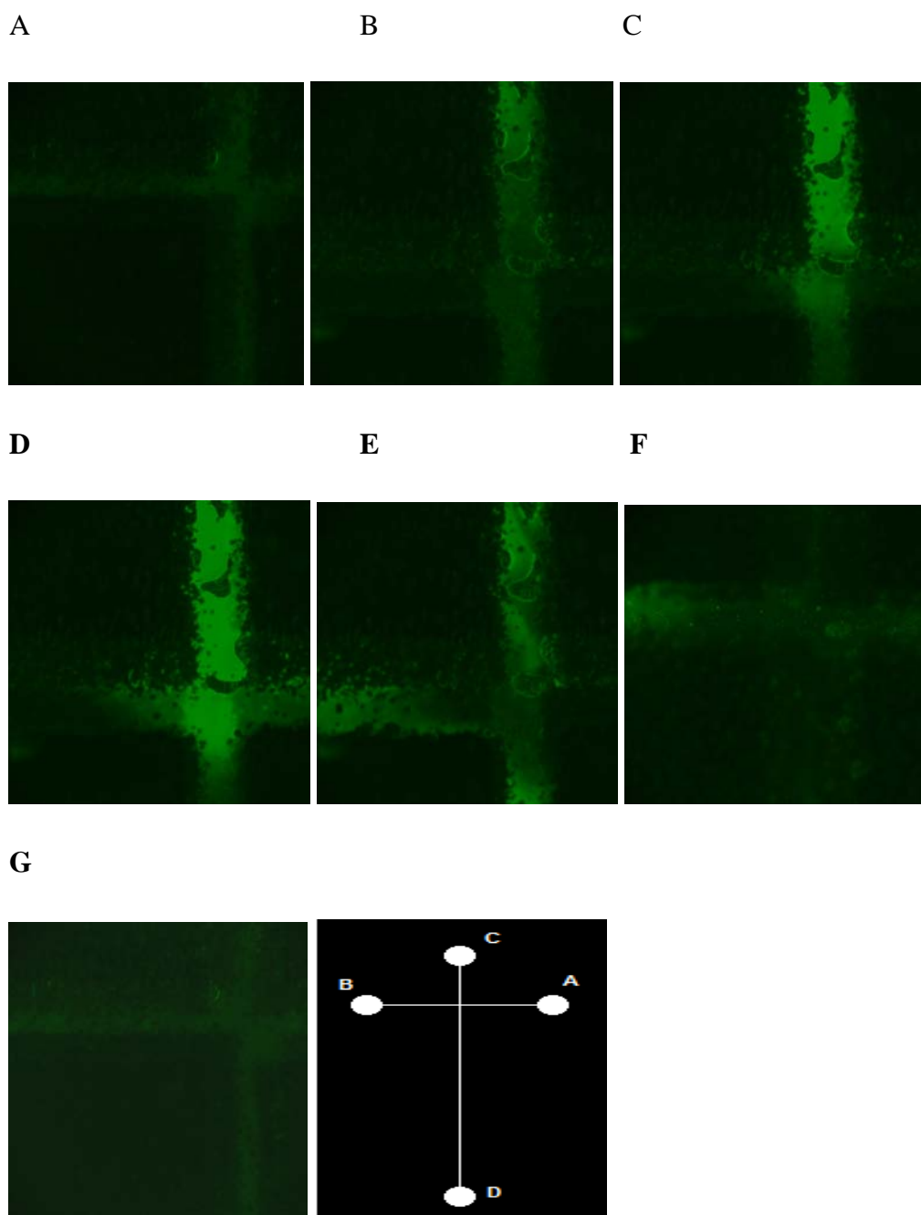
Figure 2.5: Fluorescein migrating through cross-channel of toner chip. Injection: for 25 seconds A = 200\text{ V} , B = -200\text{ V} , C = -100\text{ V} and D = -300\text{ V} . Running for 30 seconds A = 100\text{ V} , B = 100\text{ V} , C = -400\text{ V} and D = 800
