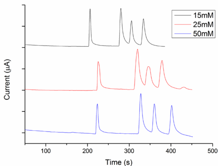
Figure 3.19: Electropherograms obtained from varying the buffer concentration. Injection buffer: varied concentration \text{Na}_2\text{B}_4\text{O}_7 \cdot 10\text{H}_2\text{O} solution, pH 9.5, and the running buffer was similar to the injection buffer with an injection time of 5 s. Acetate electrode poised at +0.9 V vs. Ag/AgCl. Concentration of analytes: 600 \mu\text{M} (each) TA, DA, Ep, NEP. Separation voltage: 10kV.
