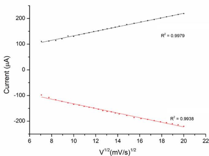
Figure 4.26: Cyclic voltammograms and the plot of the redox peak currents versus square root of the scan rate obtained at the (A) SPE and (B) SPE/CM/Au in 5 mM [\text{Fe}(\text{CN})_6]^{3-/4-} in 0.1M KCl solution at scan rate 50 to 400 mV/s.
