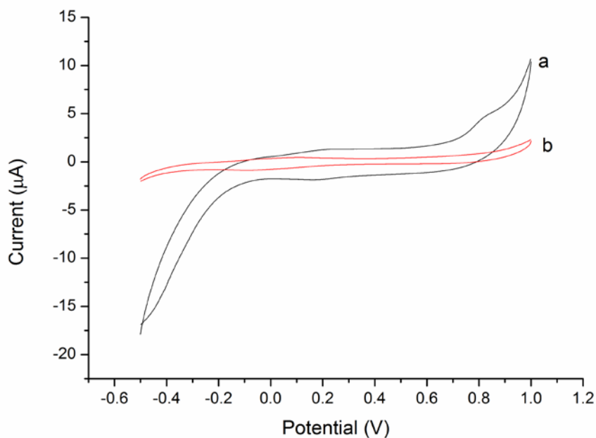
Figure 4.25: Cyclic voltammograms obtained at the (A) SPE, and (B) SPE/CM/Au in 0.1 \text{ mol L}^{-1} PB solution pH 5 at scan rate 50 \text{ mV/s} .
