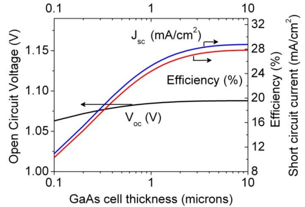
Figure 4: GaAs solar cell electrical characteristics as a function of cell thickness at T = 300 \text{ K} , 1000 \text{ W/m}^2 AM1.5d
