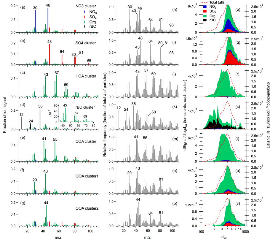
Figure 8. Normalized mass spectra (left column), normalized histograms displaying the relative frequency of each m/z (middle column), and size distributions (right column) of different clusters: (a, h and p) NO 3 cluster, (b, i and q) SO 4 cluster, (c, j and r) HOA cluster, (d, k and s) rBC cluster, (e, m and t) COA cluster, (f, n and u) OOA cluster1 – less oxygenated, (g, o and v) OOA cluster2 – more oxygenated.
