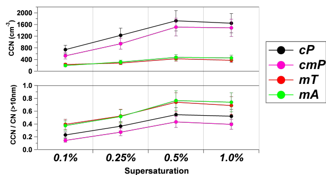
Fig. 14. (Top) CCN concentrations as a function of supersaturation and air mass classification. (Bottom) Ratio of CCN to total Condensation Nuclei at sizes larger than 10 nm diameter.
