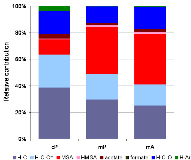
Fig. 12. 1H NMR chemical characterization of WSOC as a function of the air mass origin
