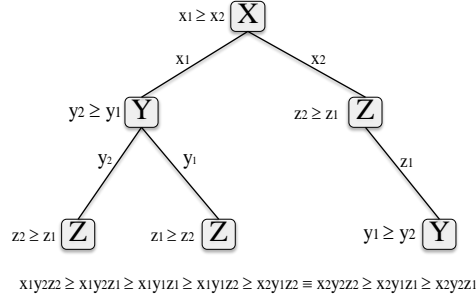
Fig. 1. A cp-tree \sigma , along with its associated ordering \succ_{\sigma} on outcomes, with \gamma = 1 (i.e., with at most one variable associated with a node)
