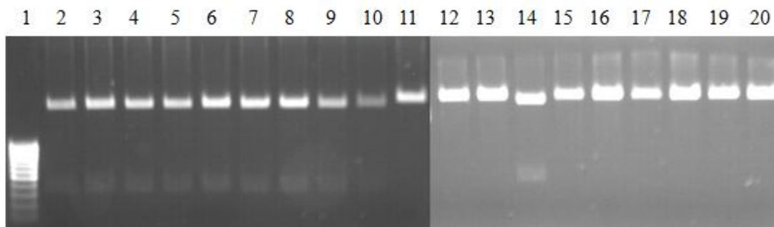
Figure 5.4: Digest analysis of clones derived from golden gate cloning of CRISPR gRNAs into pEXA. Lane 1: Low range Ladder. Lanes 2-11: Potential clones derived from CRISPR in9 ligation. Lanes 12-20: Potential clones derived from CRISPR ex10 ligation. Successful cloning produces a single band as seen in lane 11 and in all lanes except 14 in lanes 12-20.
