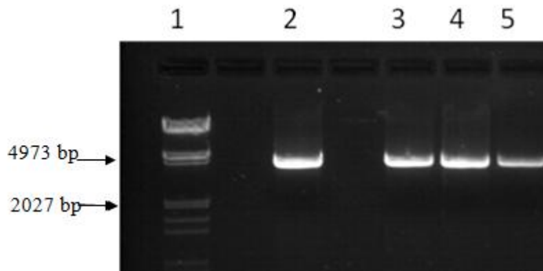
Fig 3.1: Temperature optimisation of CFTR-Fwd- BstEII and CFTR-Rev- MluI primers. Lane 1: EcoRI/HindIII lambda ladder, band sizes 2027 and 4973 bp indicated by arrows. Lanes 2-5: 20µl PCR product of genomic HBE DNA at 51.6, 56.8, 54, 60 °C.
